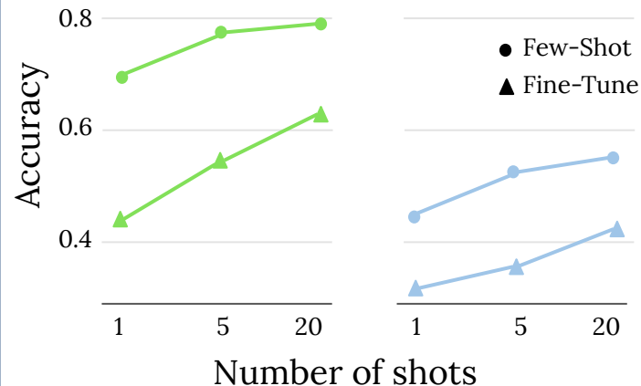
Few Shot performances on Tests sets
