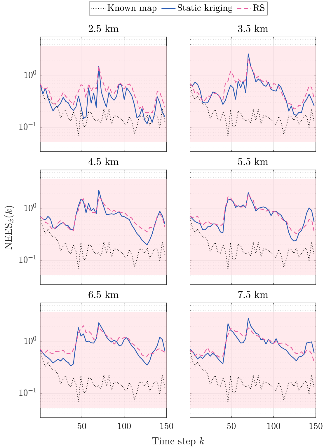
Figure 4.11: Comparative NEES of the navigation algorithms using static kriging or random subsampling across the six grid resolutions. The shaded area corresponds to that of the previous NEES figure.
