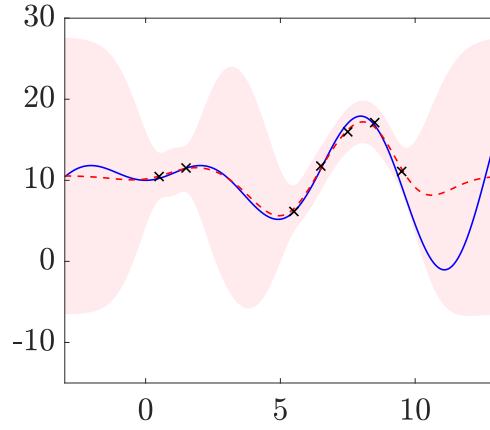
Figure 4.2: Simultaneous kriging of the training data and mean estimation by ordinary kriging. The constant mean is reconstructed here at \hat{m}_{\text{OK}} = 10.56 .
