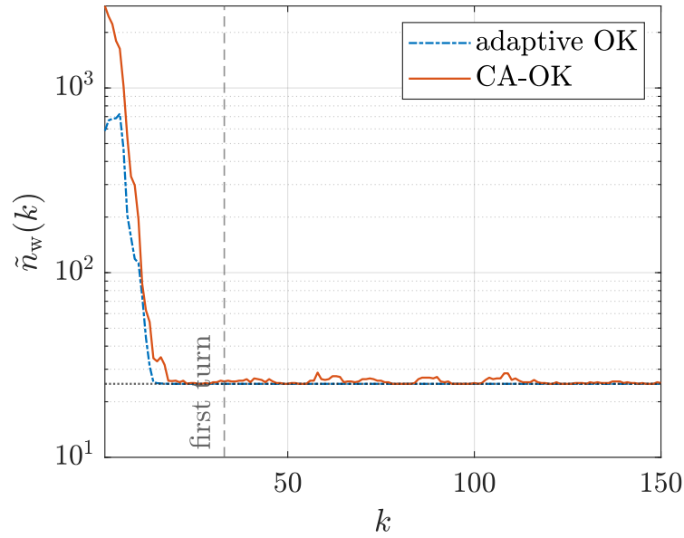
Figure 4.10: Samples retained per query along the flight. The dotted line is the floor n_{\min} , and the dashed one marks the first half-turn.
