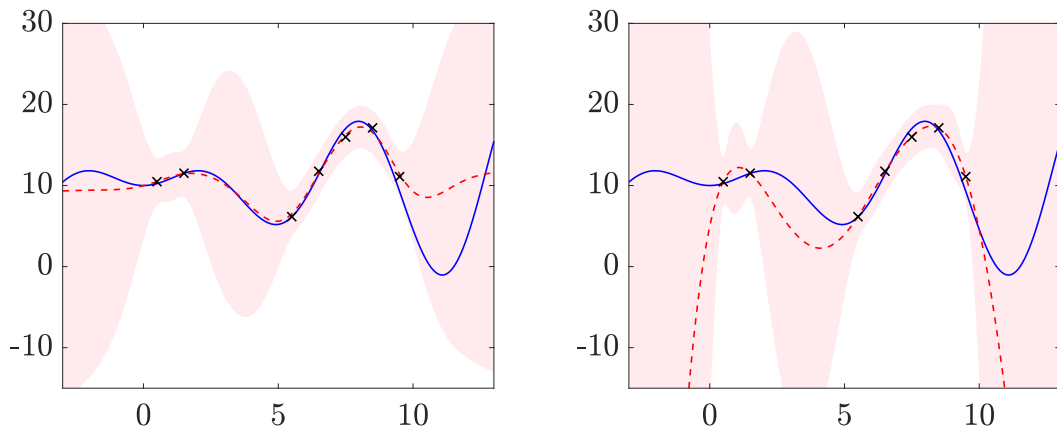
Figure 4.3: Universal kriging over an affine trend basis, on the left, and over a degree five monomial basis, on the right. The trend coefficients are estimated here at \hat{m}_{\text{UK}} = [9.78, 0.15]^\top and \hat{m}_{\text{UK}} = [4.95, 15.85, -10.82, 2.40, -0.20, 0.01]^\top respectively.
