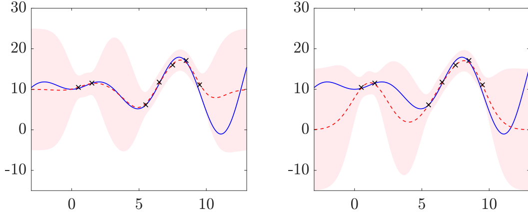
Figure 4.1: Simple kriging under a correct mean function, on the left, and under a wrong one, on the right. Since R_{\text{SK}} does not depend on m in (3.35), both shaded areas have the same width along the x -axis.
