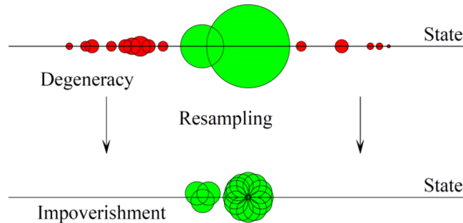
Figure 2.3: Particle impoverishment after resampling. Discarding non-resampled particles progressively shrinks the support of the particle approximation, degrading the filter’s ability to explore the state-space.
