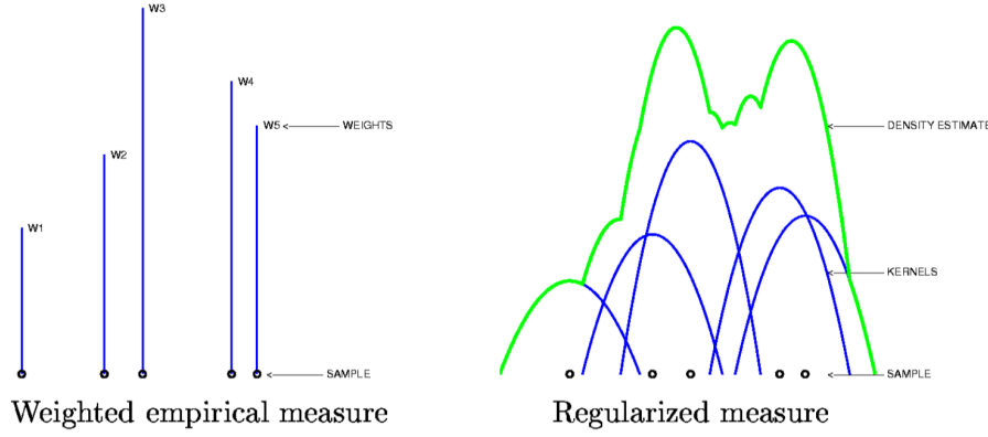
Figure 2.4: An example Monte Carlo approximation of the PDF (2.122) on the left and its kernel regularisation (2.123) on the right, for a given particle set. The latter approximation bridges the gaps between particles and spans a larger region of the state space.
