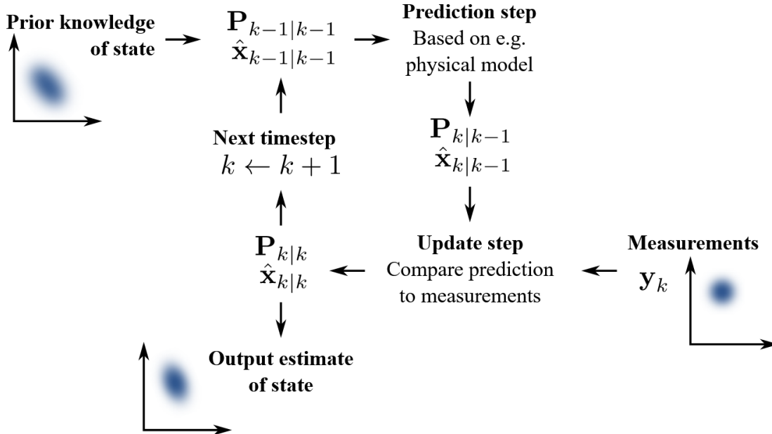
Figure 2.1: Schematic representation of the Kalman filter prediction/correction cycle. Each ellipsoid represents a confidence region associated with its corresponding Gaussian density.
