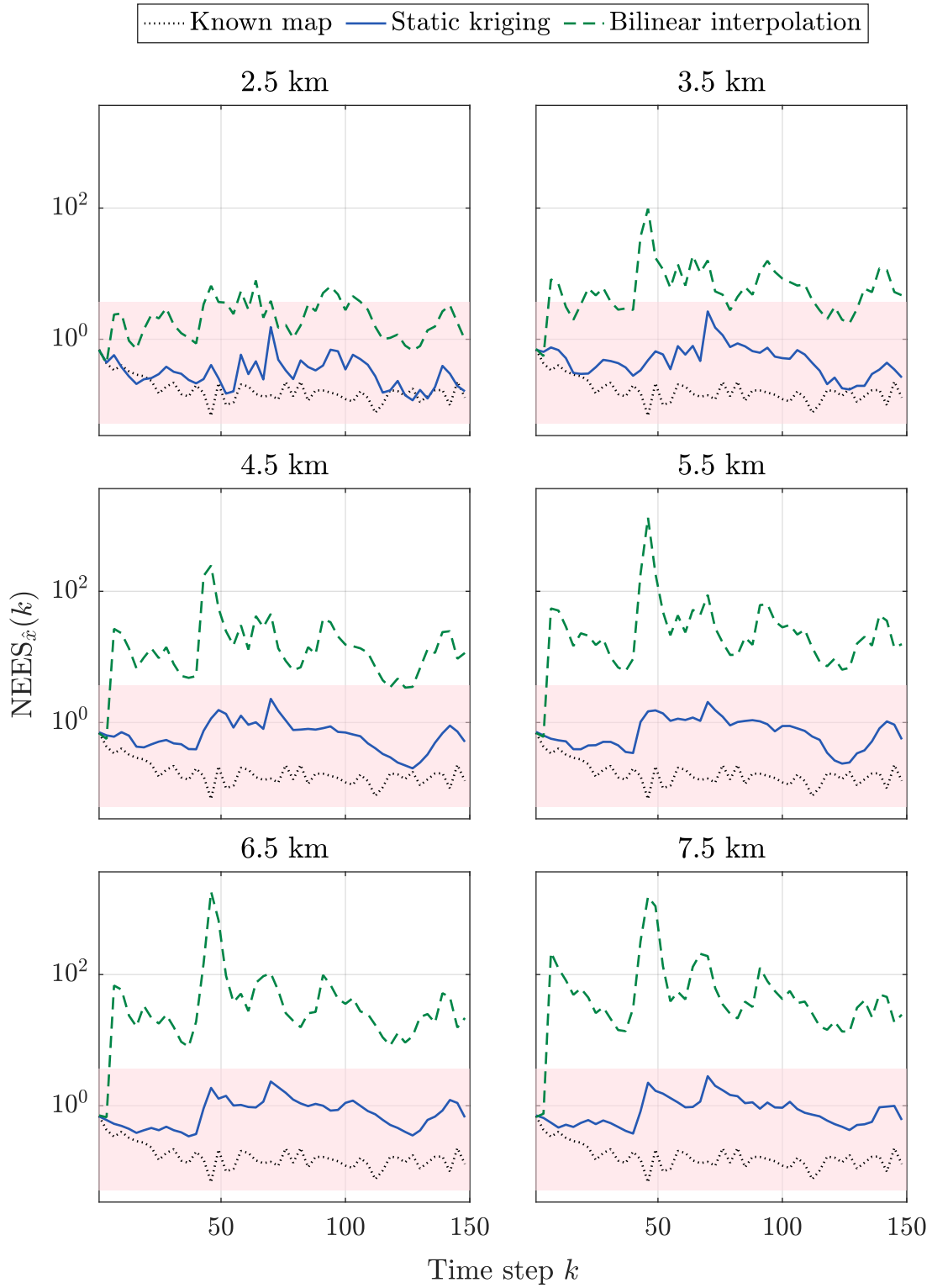
Figure 4.7: Estimation NEES of the navigation algorithms using the known map, bilinear interpolation and static kriging. The shaded area delimits the quantiles of a \chi^2 law with d_x degrees of freedom, within which the NEES of a consistent filter falls with probability 0.99.
