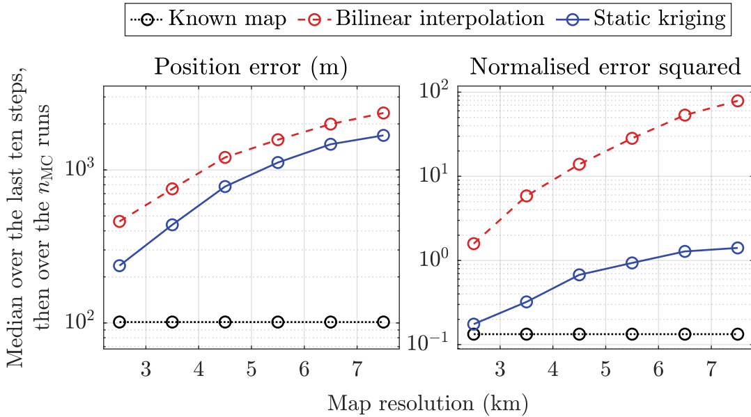
Figure 4.8: Average median RMSE and NEES at the end of the flight for each grid resolution. These metrics are used to determine whether a run has converged.
