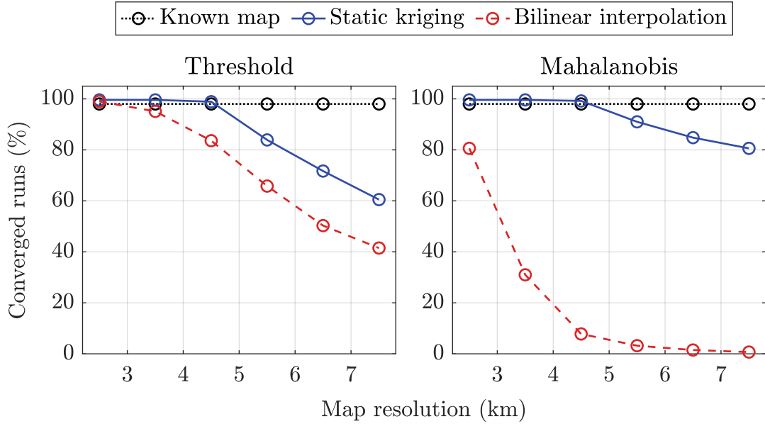
Figure 4.9: Percentage of converged runs against the grid resolution for the two metrics. The true map does not depend on the resolution, and has a convergence rate of 98% under both criteria.
