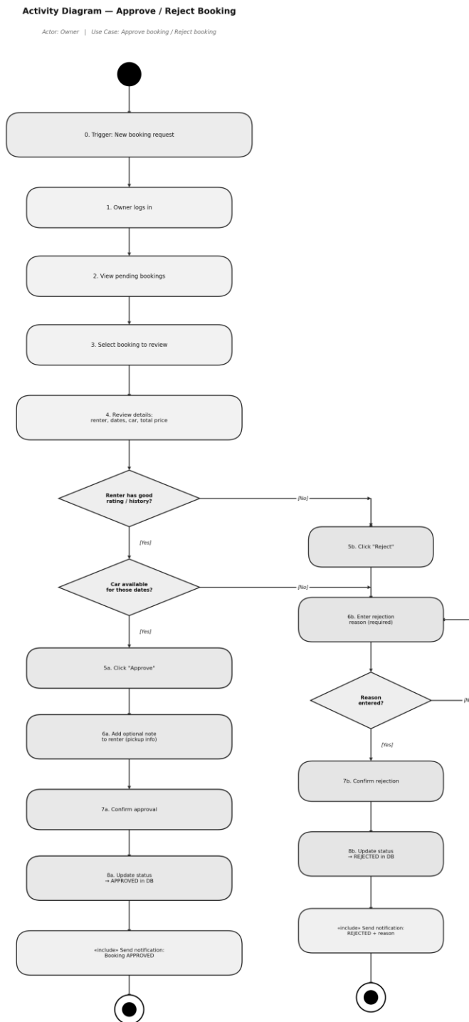
Figure 7: Activity Diagram for approving or rejecting a booking
