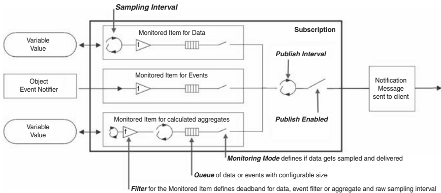
Fig. 5.9 Settings for Subscription and Monitored Items
