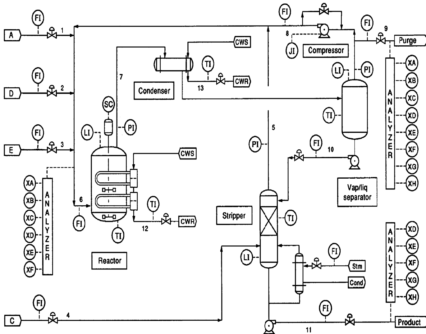
Fig. 1. Tennessee Eastman test problem.
