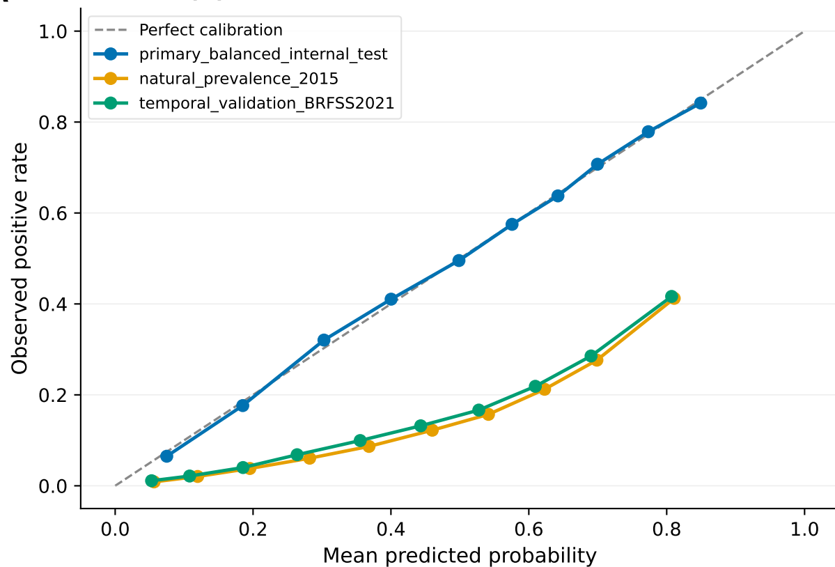
(A) Calibration curves — all evaluation sets
