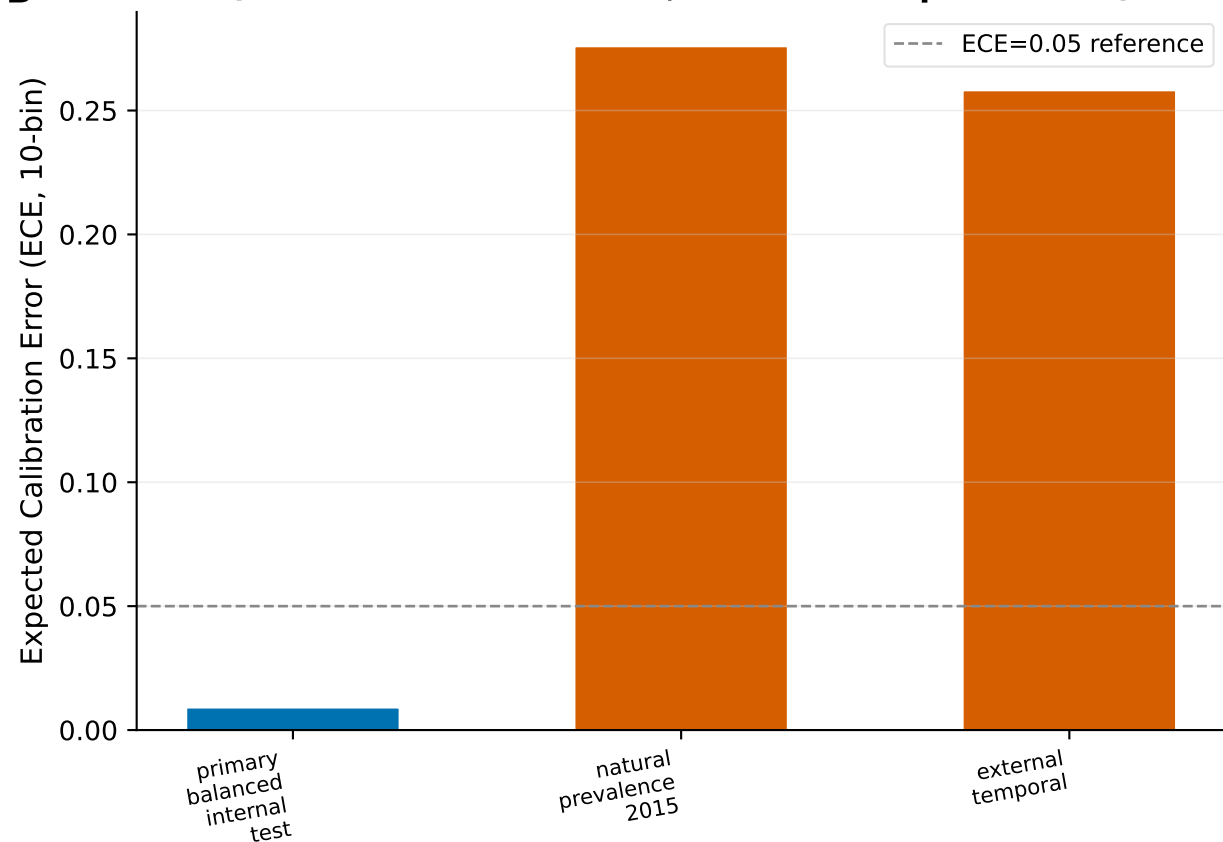
(B) ECE by evaluation set (blue=balanced internal; red=natural prevalence)
