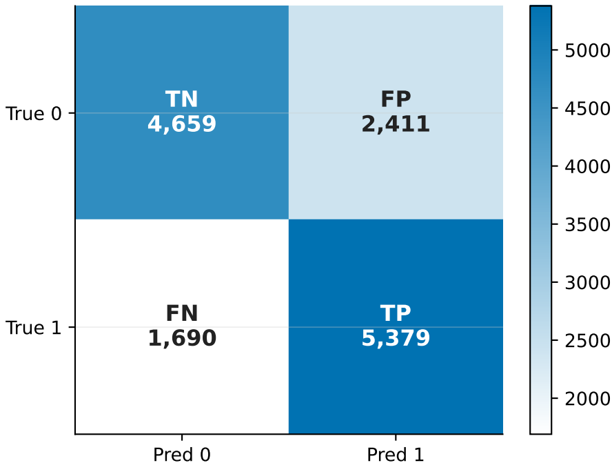
Confusion matrix — default threshold 0.50
