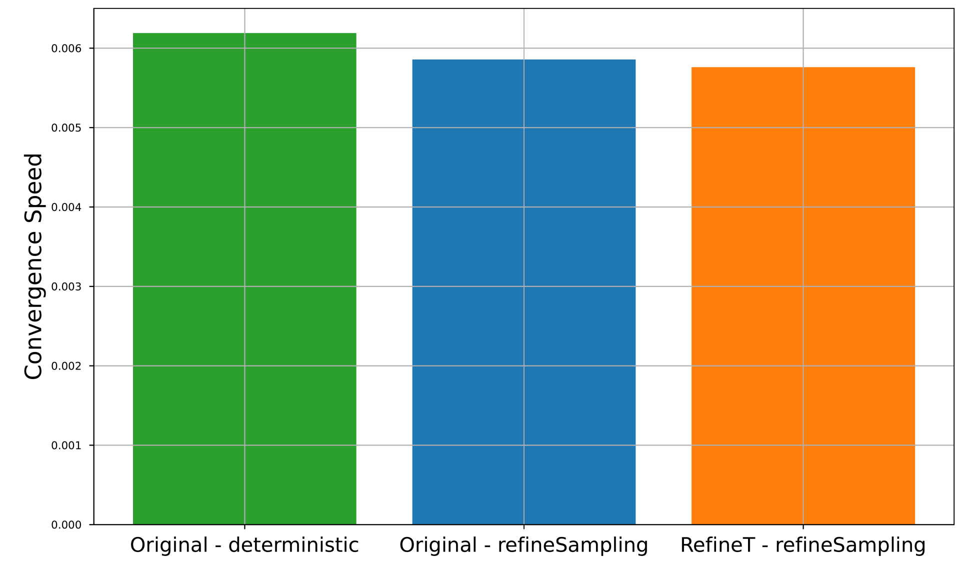
(f) Reacher-v4
