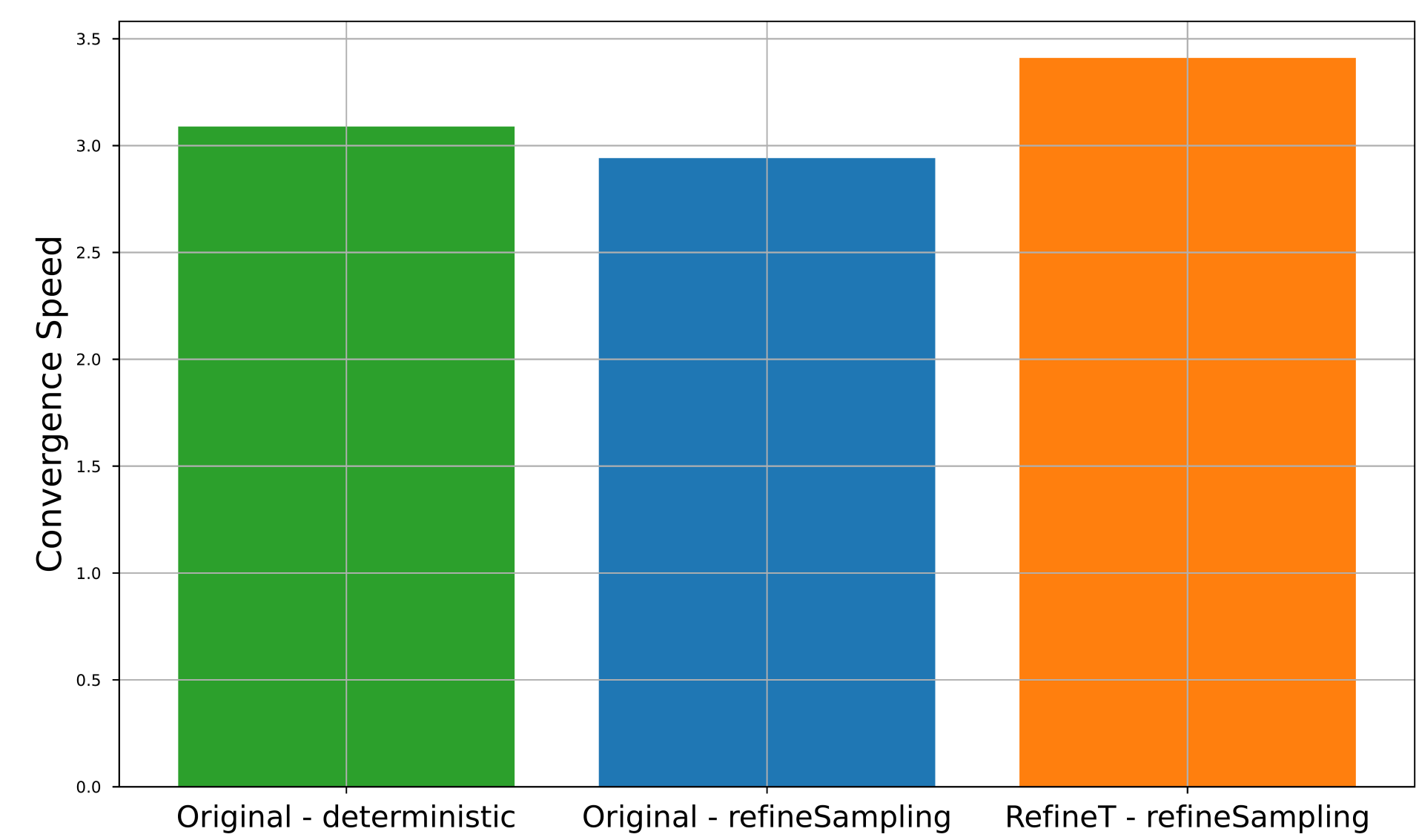
(c) Hopper-v4
