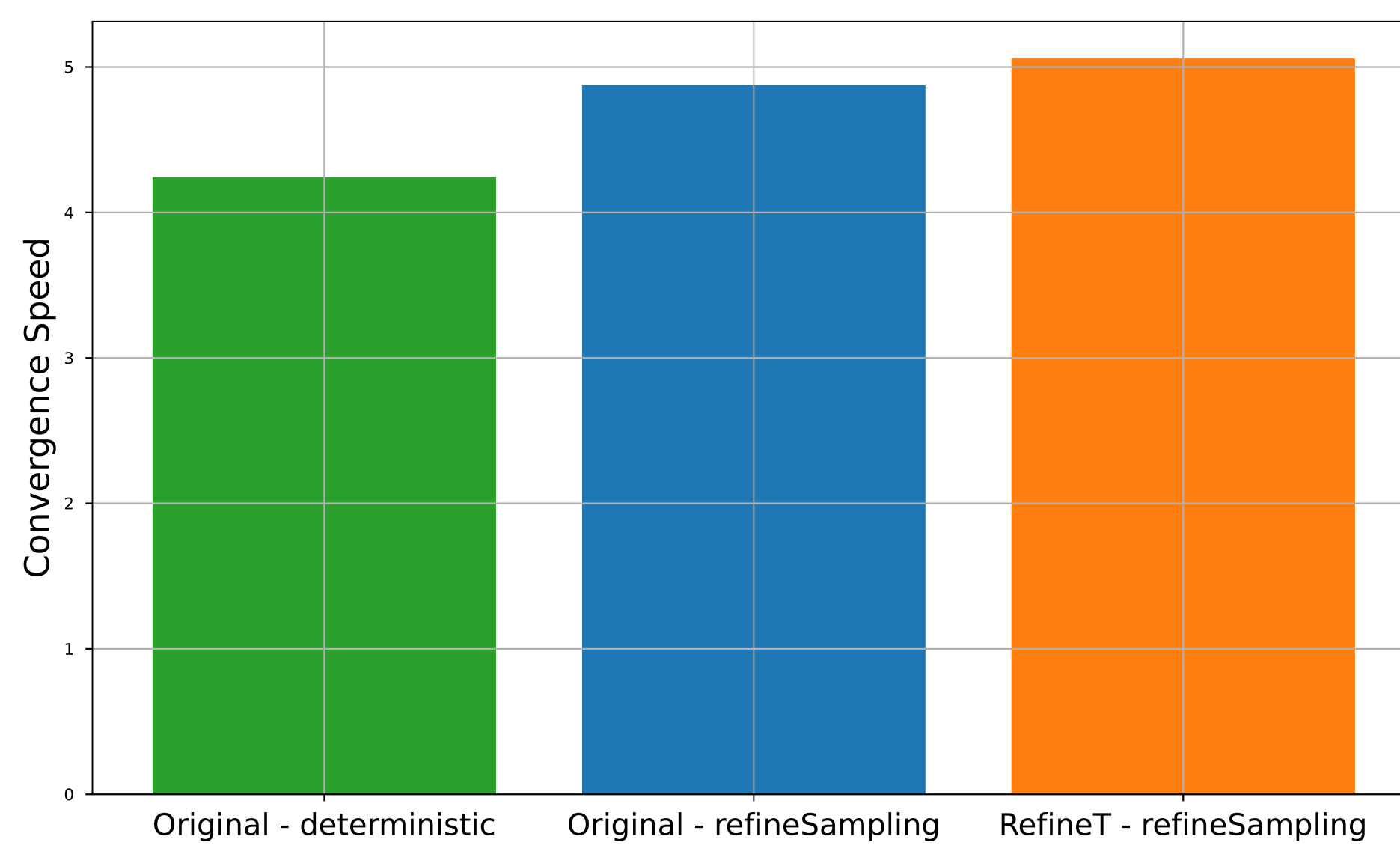
(a) Humanoid-v4
