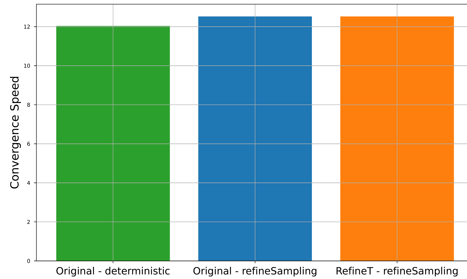
(e) HalfCheetah-v4
