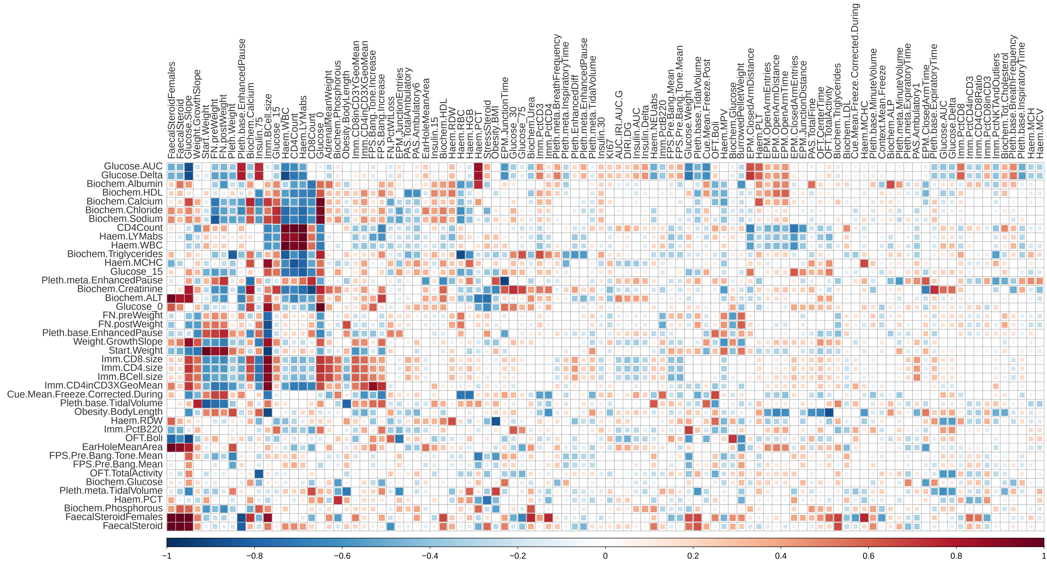
corr_Ad2s1 – significance: p(fdr)<0.1: * – HSmice
