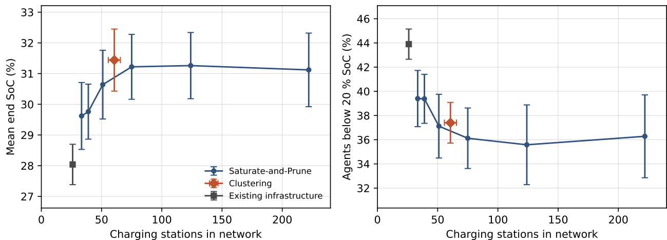
Figure 4: Accessibility against number of charging stations, mean over five scenario seeds with standard deviation as error bars. Left: mean SoC of the fleet at the end of a simulated day. Right: share of agents ending below 20% SoC. The line traces successive prune iterations of Saturate-and-Prune. Clustering produces its network in a single pass.
