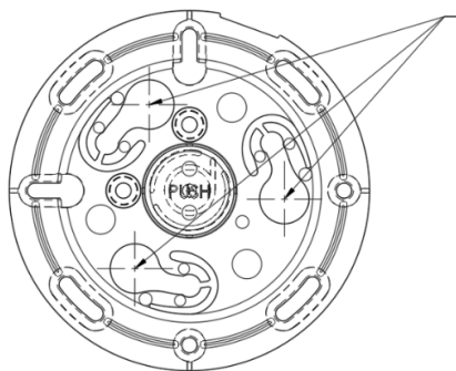
Figure 6.3-3: Top view of the mounting plate showing the snap-fit fittings
