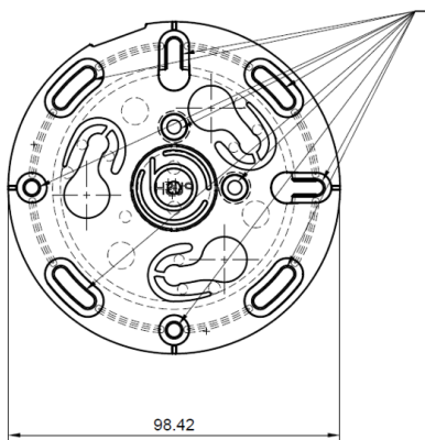
Figure 6.3-2: Top view of the mounting plate showing the mounting points
