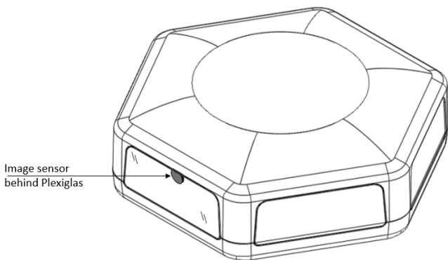
Figure 3.1-1: View of the device showing the built-in camera (without mounting plate)
