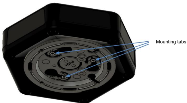
Figure 6.3-4: Bottom view of the mounting plate with the Eyepatch attachment fixed in place. Figure 6.3-4 shows the device's three locking tabs, which are positioned at the end positions of the locking recesses in the mounting plate (connected and locked).
