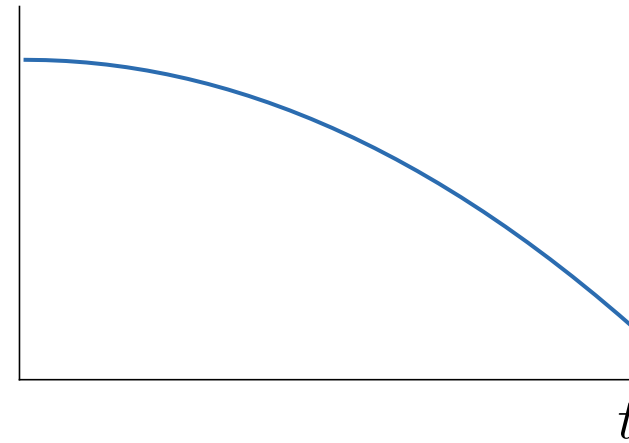
LocalAcceleration
