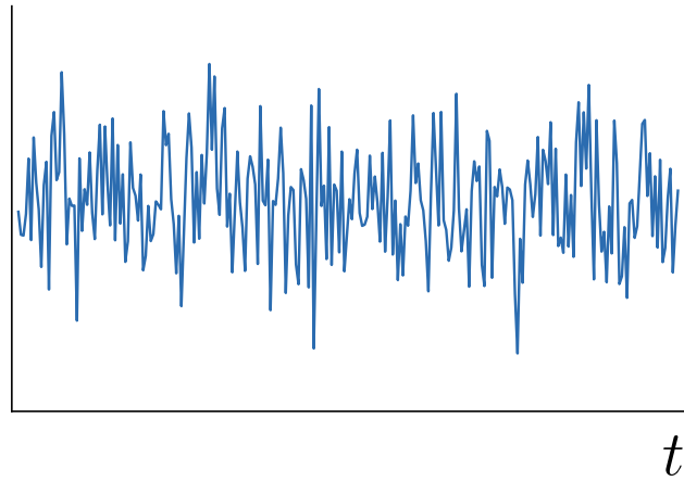
WhiteNoise
