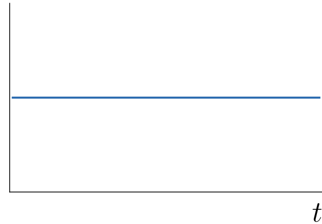
LocalLevel
