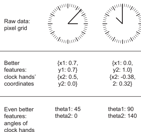
Figure 4.3 Feature engineering for reading the time on a clock
