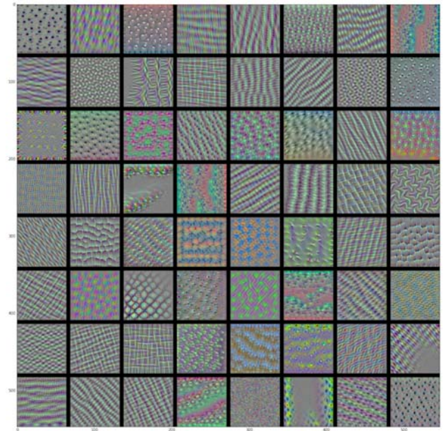
Figure 5.32 Filter patterns for layer block3_conv1
