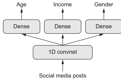
Figure 7.7 A social media model with three heads
