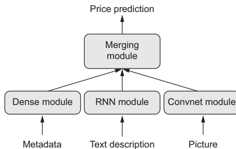
Figure 7.2 A multi-input model
