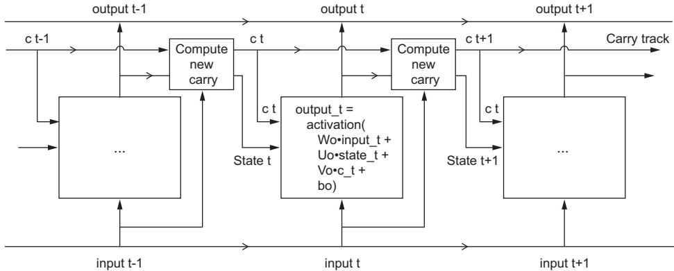
Figure 6.15 Anatomy of an LSTM
