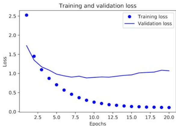
Figure 3.9 Training and validation loss
