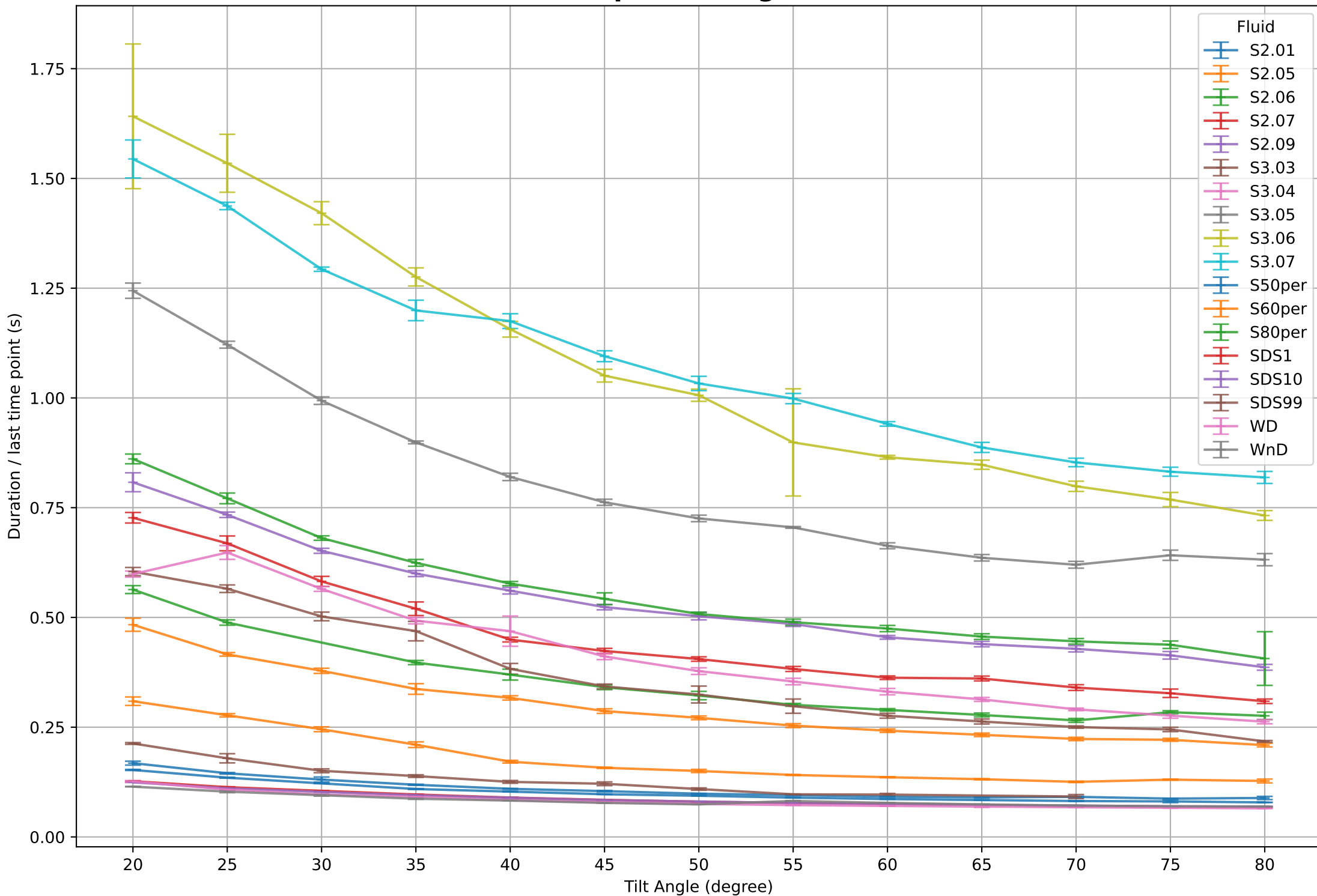
Mean duration per tilt angle for each fluid
