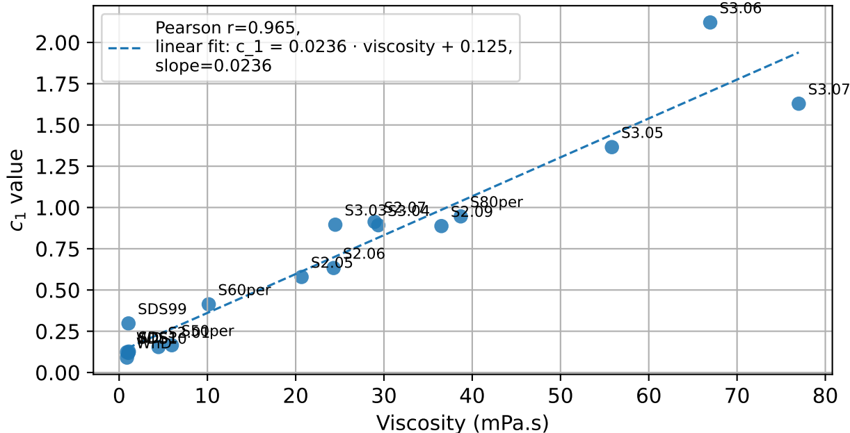
best_model_0: correlation between viscosity and c_1 Pearson r=0.965 , Spearman r=0.959
