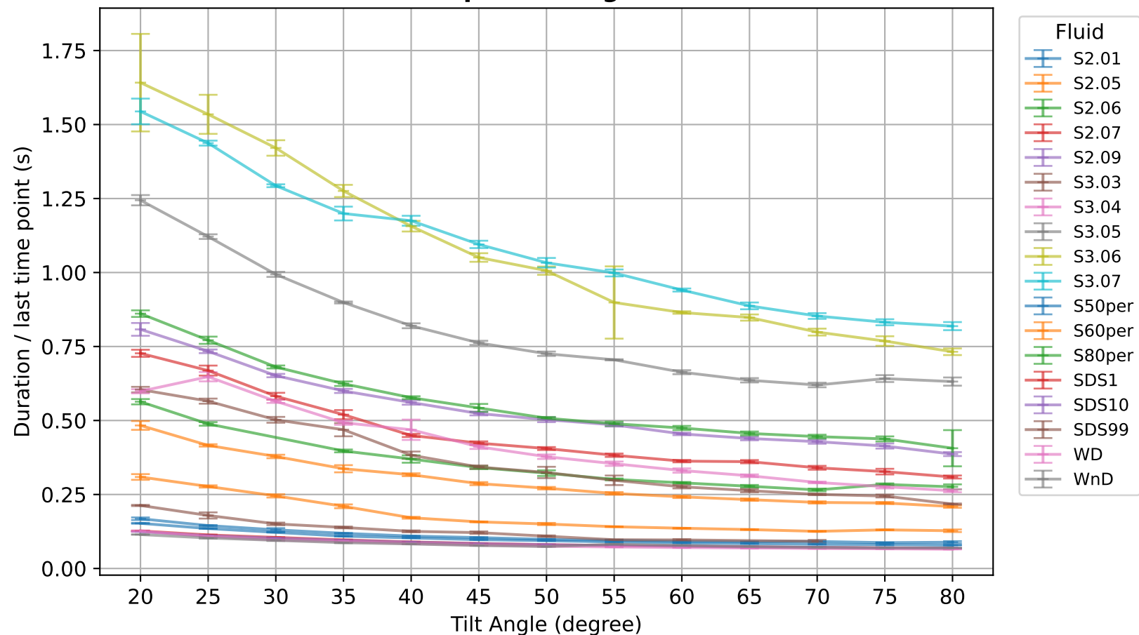
Mean duration per tilt angle for each fluid
