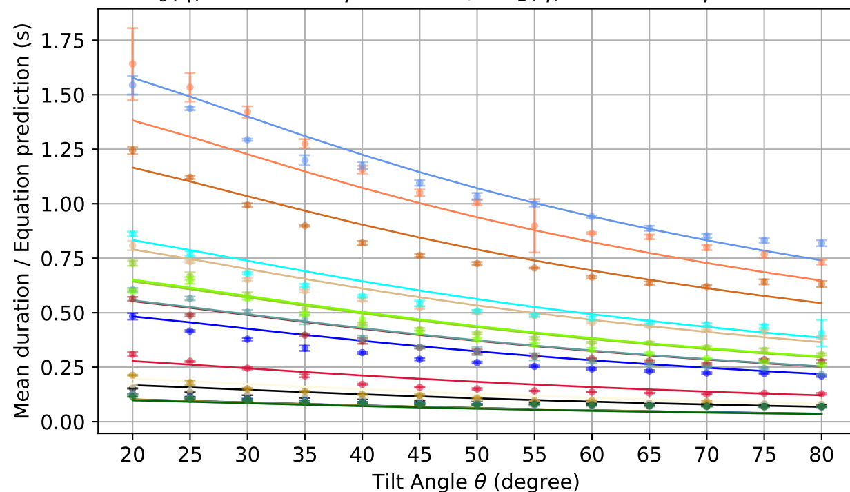
Original best_model_0 with fitted fluid-specific constants
