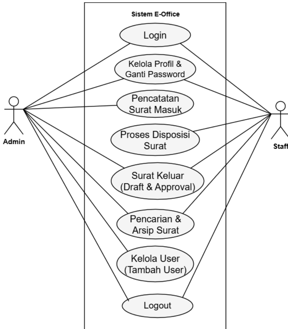
Gambar 3.4 Diagram Use case
