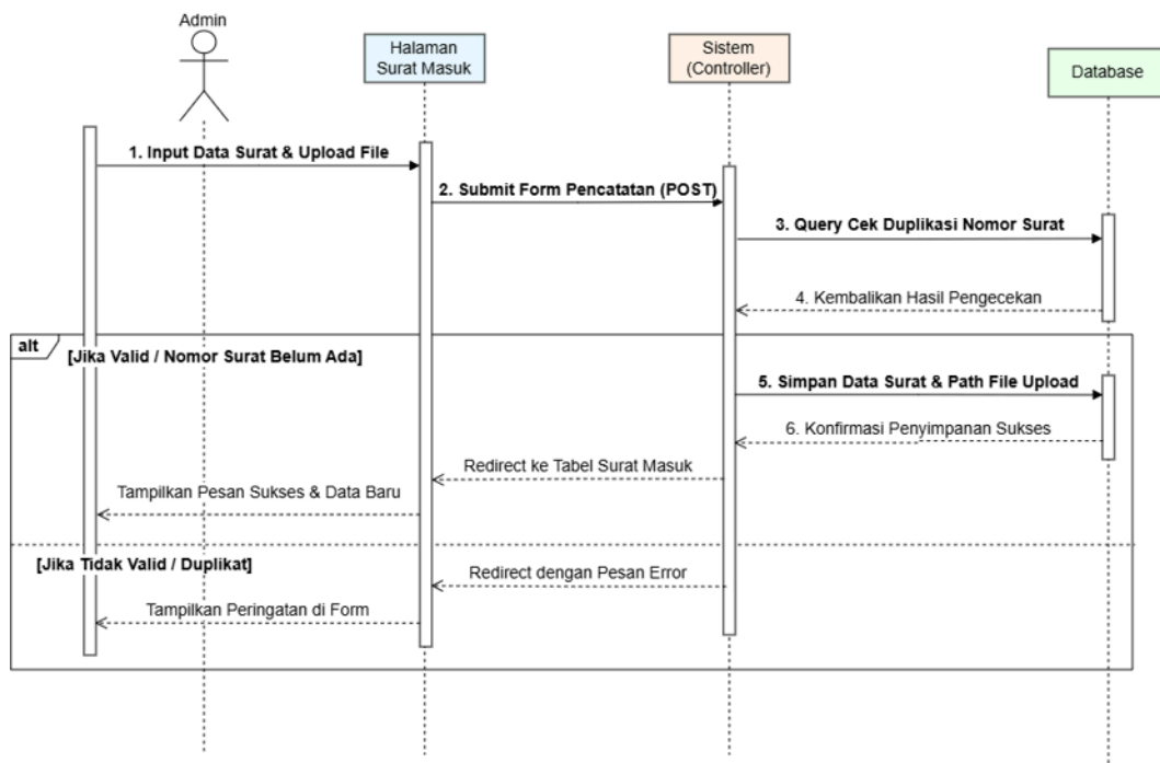
Gambar 3.15 Sequence Diagram Pencatatan Surat Masuk
