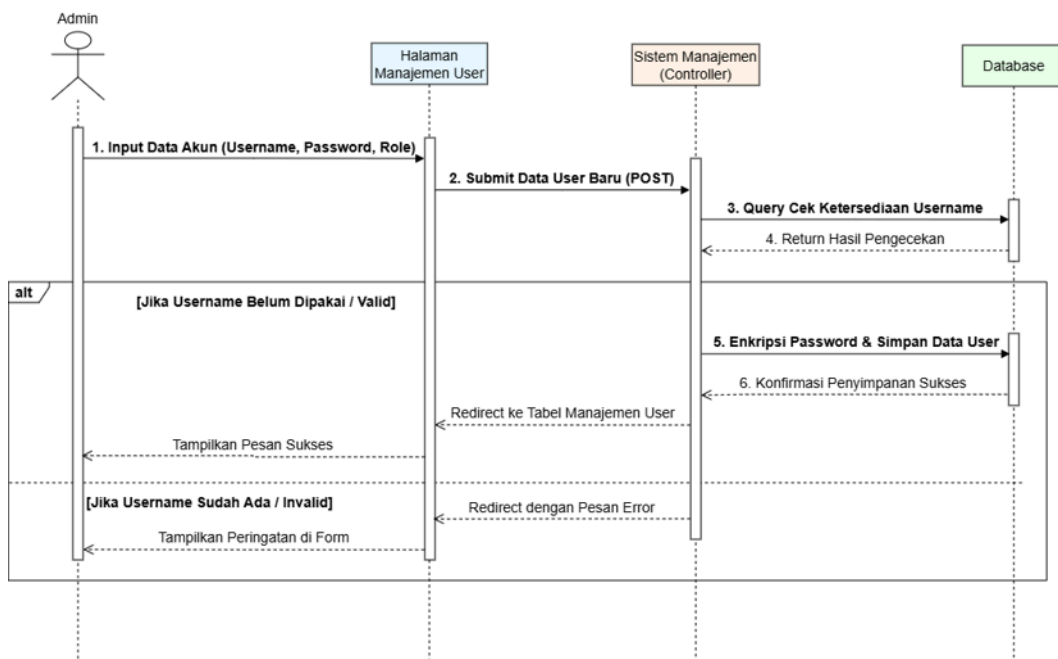
Gambar 3.19 Sequence Diagram Kelola User (Tambah User)
