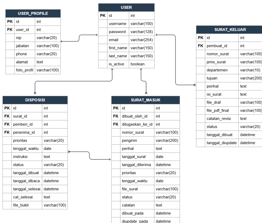
Gambar 3.22 Entity Relationship Diagram (ERD)
