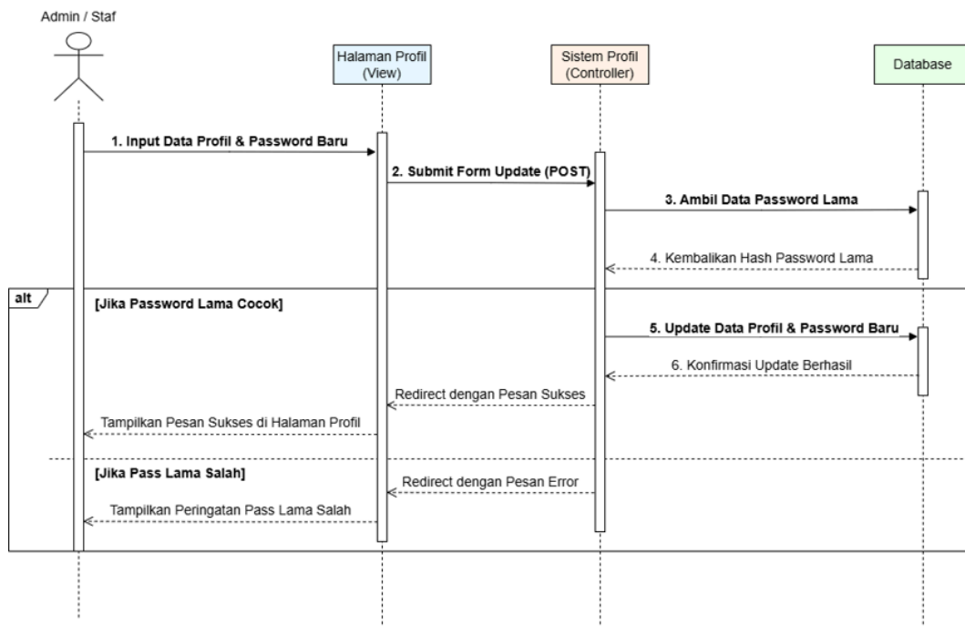
Gambar 3.14 Sequence Diagram Kelola Profil & Ganti Password
