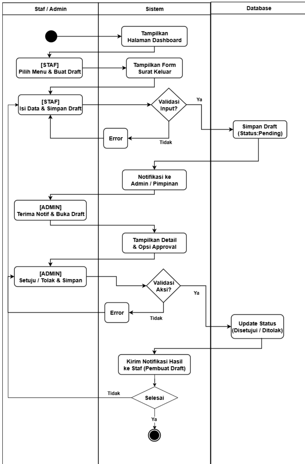
Gambar 3.9 Activity Diagram Surat Keluar (Draft & Approval)
