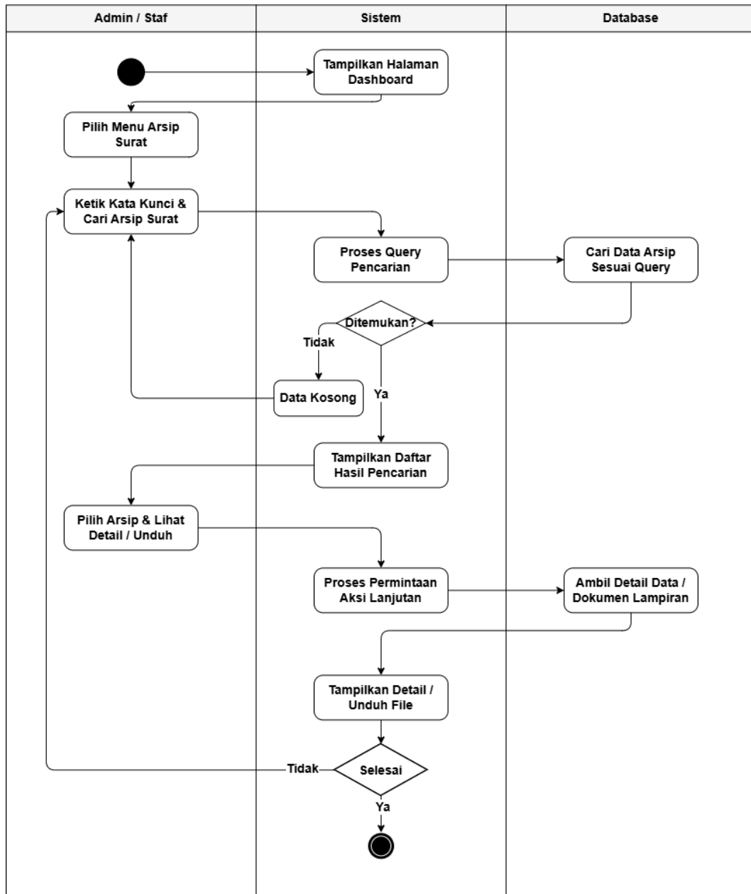
Gambar 3.10 Activity Diagram Pencarian & Arsip Surat
