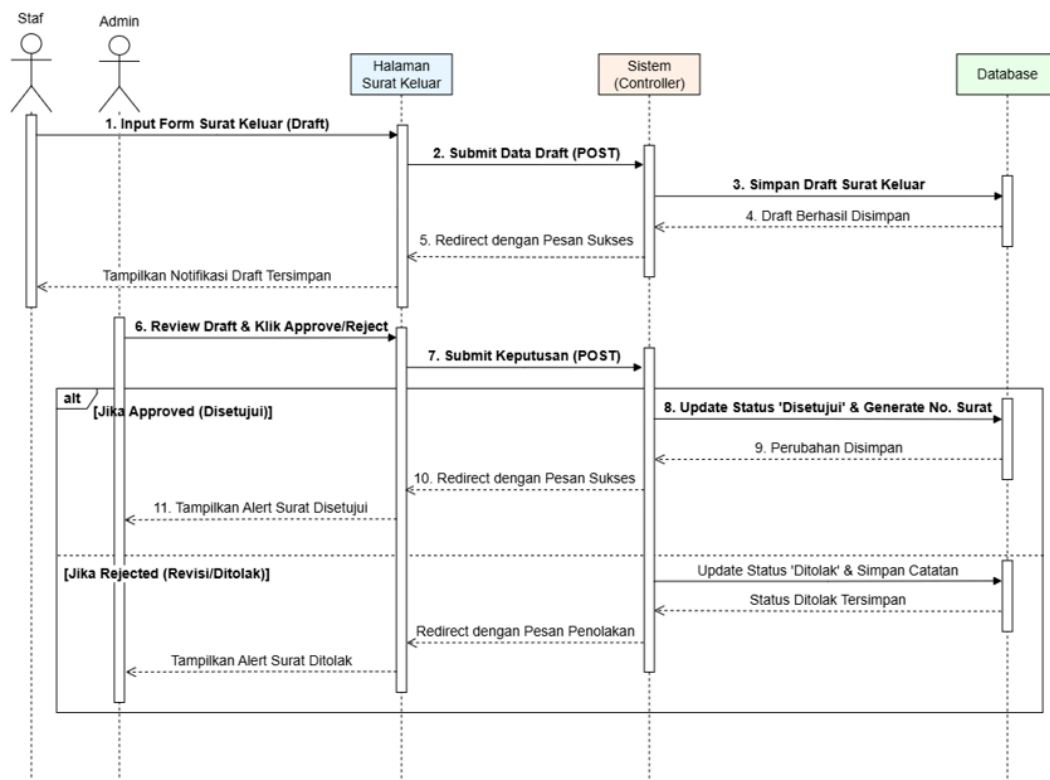
Gambar 3.17 Sequence Diagram Surat Keluar (Draft & Approval)
