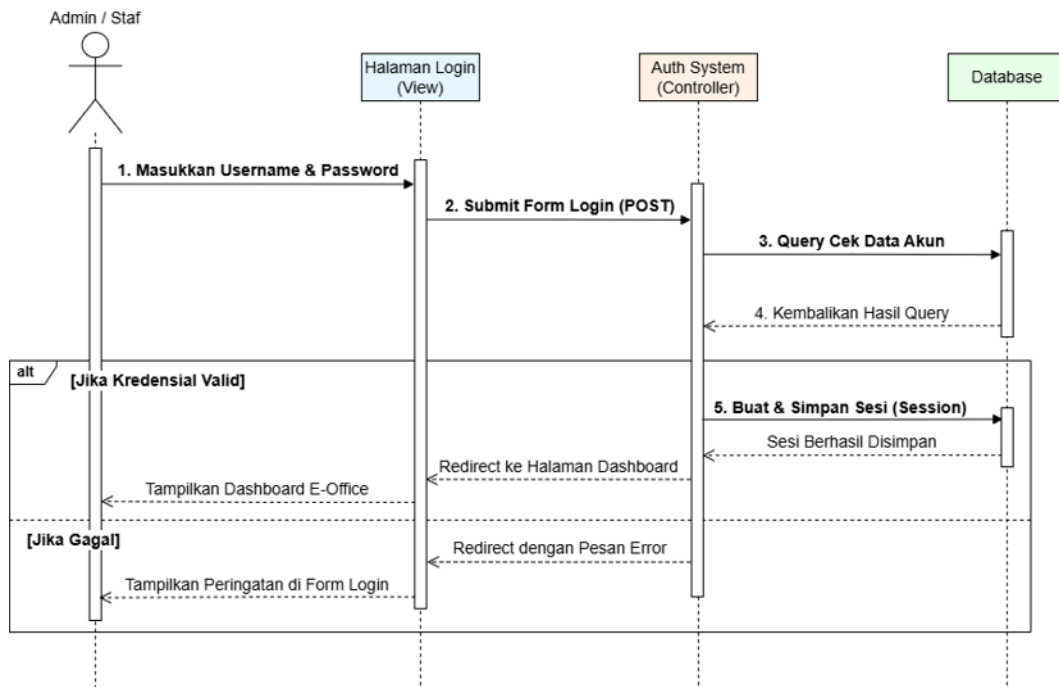
Gambar 3.13 Sequence Diagram Login
