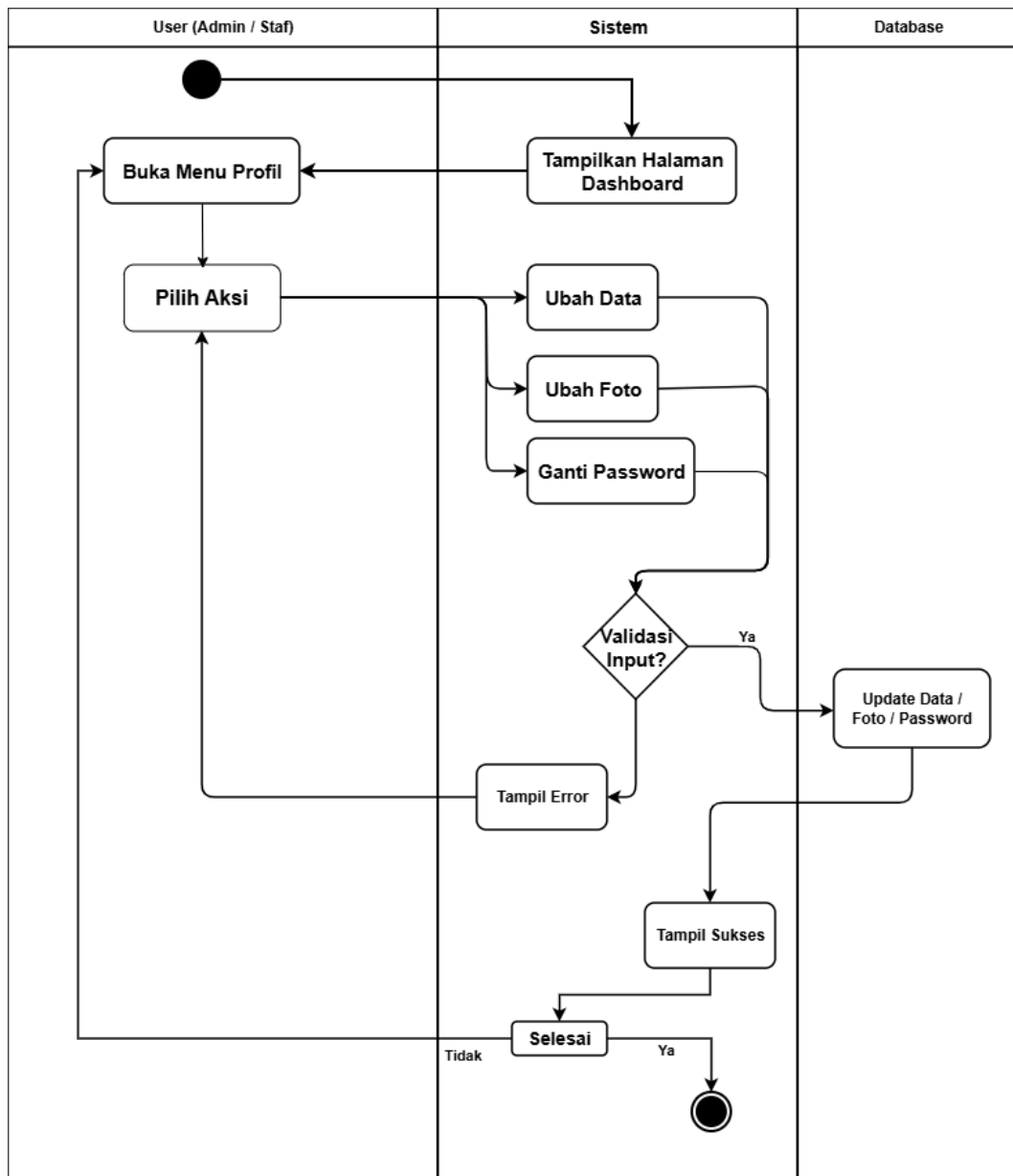
Gambar 3.6 Activity Diagram Kelola Profil & Ganti Password
