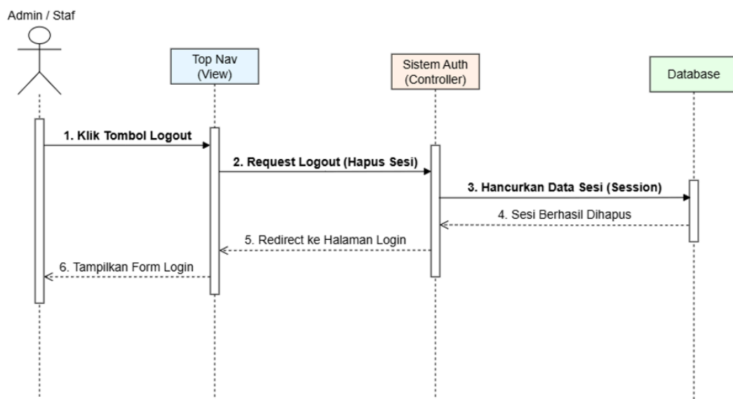
Gambar 3.20 Sequence Diagram Logout
