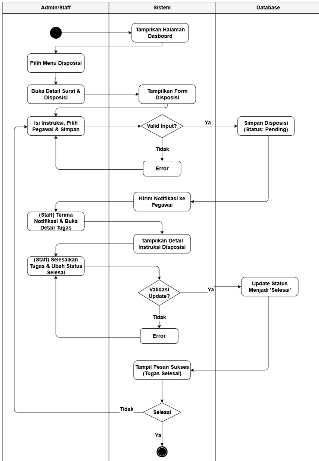
Gambar 3.8 Activity Diagram Proses Disposisi Surat
