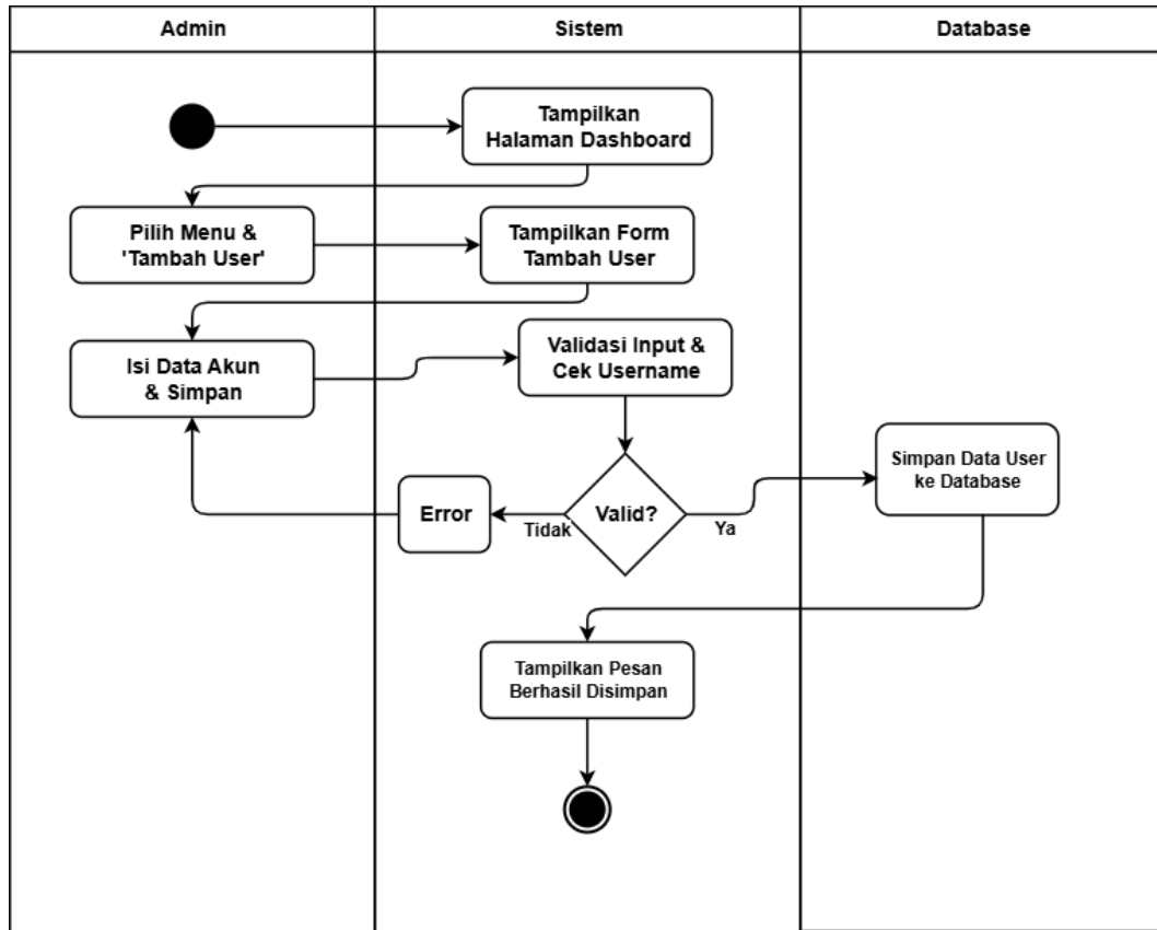
Gambar 3.11 Activity Diagram Kelola User (Tambah User)
