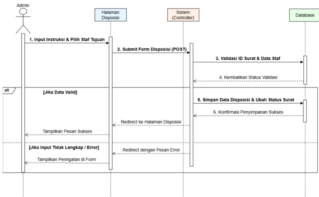
Gambar 3.16 Sequence Diagram Proses Disposisi Surat
