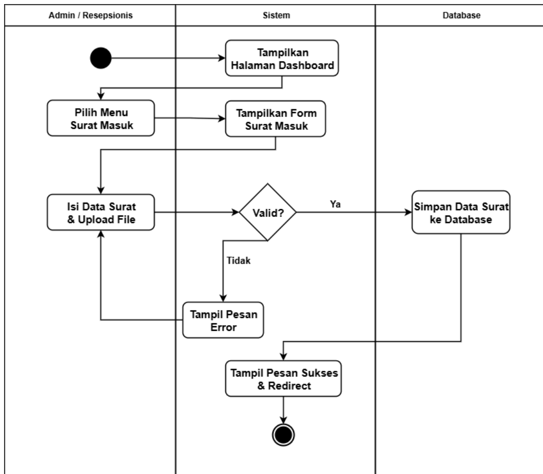
Gambar 3.7 Activity Diagram Pencatatan Surat Masuk
