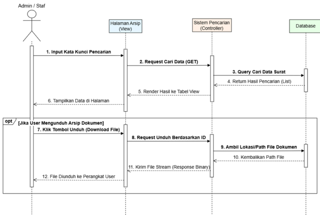
Gambar 3.18 Sequence Diagram Pencarian & Arsip Surat
