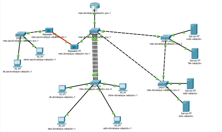
Рис. 9: EtherChannel
