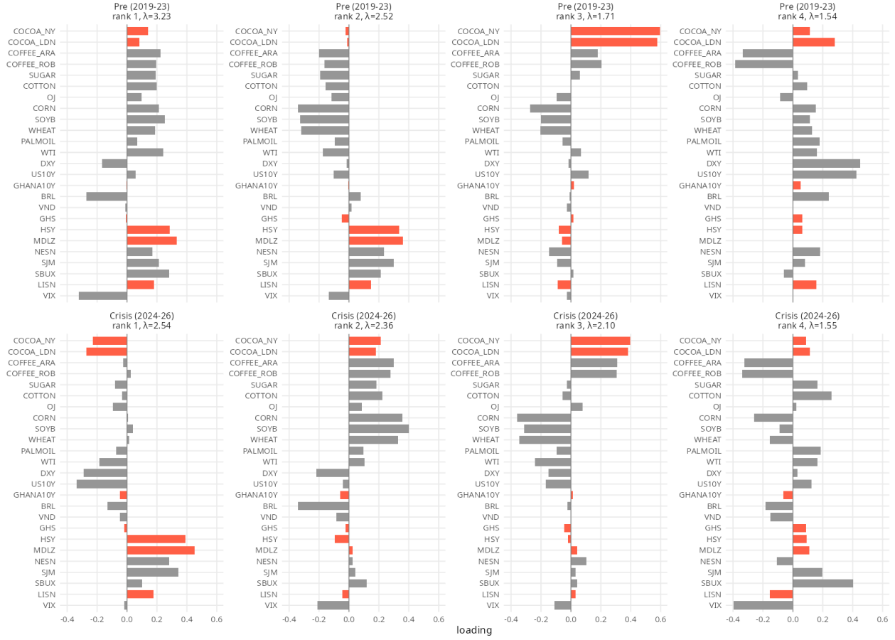
Figure 2: Eigenvector loadings of the top four supra-MP eigenvalues, pre-crisis (top row) vs in-crisis (bottom row), sign-normalised. Red bars: cocoa bloc {COCOA_NY, COCOA_LDN, HSY, MDLZ, LISN, GHS, GHANA10Y}. The rank-1 in-crisis mode (the market mode) reorganises to put cocoa contracts and chocolate-maker equities jointly on it.
