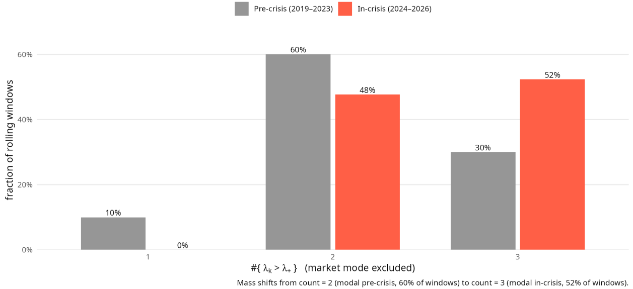
Figure 1: Distribution of the rolling 252-day supra-MP eigenvalue count (market mode excluded), pre-crisis (2019–2023, grey) vs in-crisis (2024–2026, red). The modal count shifts from 2 (60% of pre-crisis windows) to 3 (52% of in-crisis windows); the count = 1 mass present pre-crisis (10%) disappears entirely in crisis.
