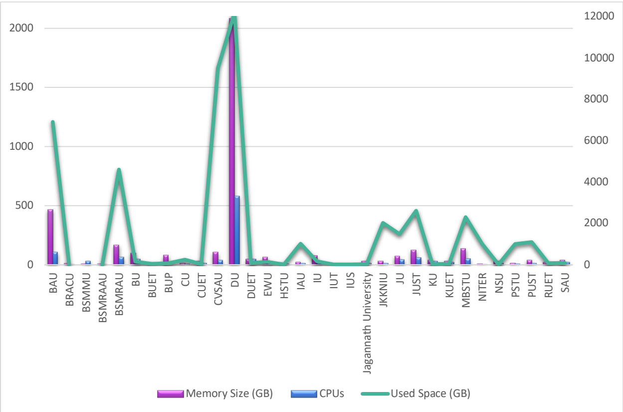
Figure 8: Institution Wise Max HPS Usage
