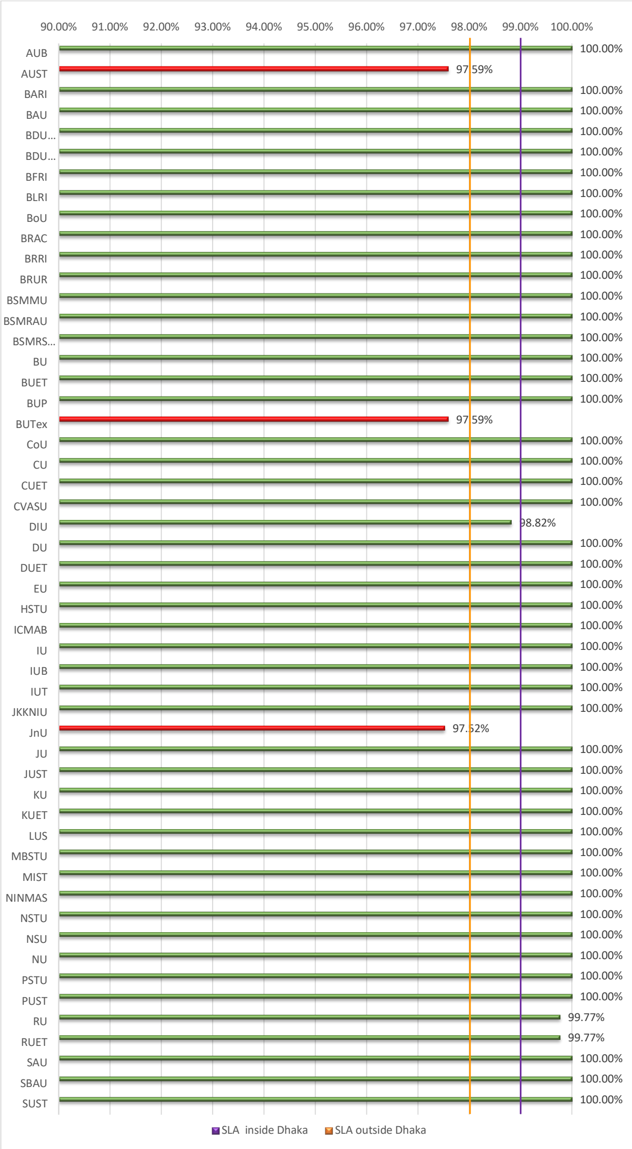
Figure 2: Institution Wise Link Availability considering “Planned Maintenance” as outage
