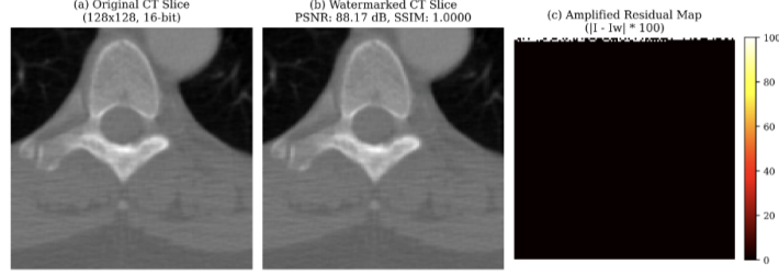
Fig. 3. Visual fidelity comparison on a 128 \times 128 sample demonstrating (a) original matrix, (b) watermarked slice, and (c) amplified difference map ( |I - I_w| \times 100 ). Note: localized 88.17 dB PSNR differs from full-scale evaluations in Table 2.
