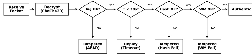
Fig. 1. Logical architecture and decision flow of the receiver verification stage, illustrating the sequential cryptographic and provenance checks.
