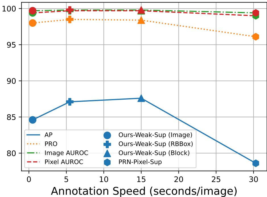
AD Performance
