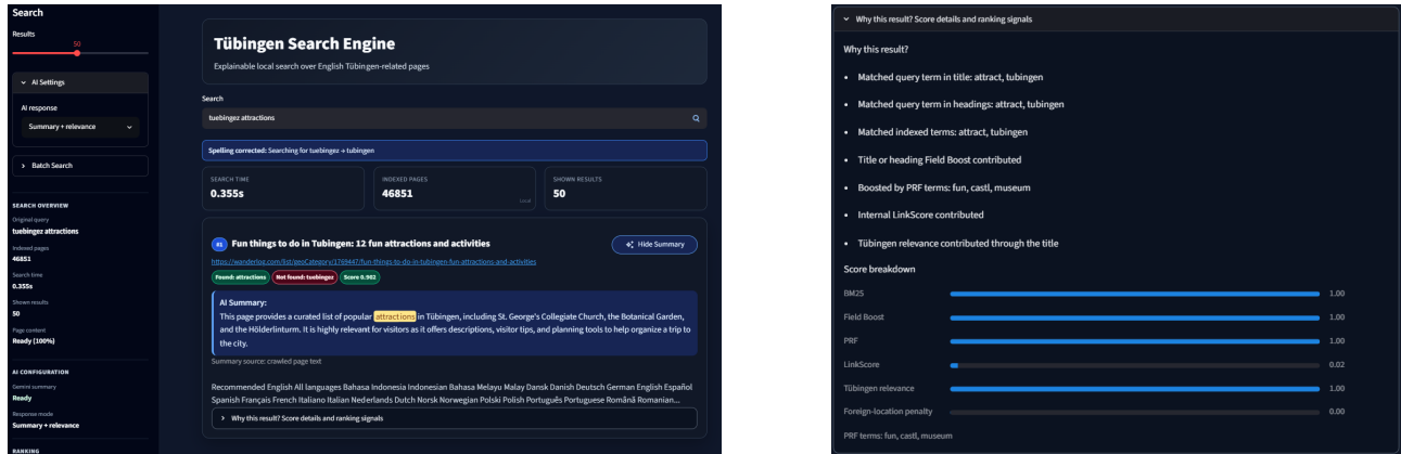
Figure 1. Search interface showing spelling correction, Found and Not found query-term badges, and an AI-generated result summary (left), and the expanded ranking explanation with its score breakdown (right).
