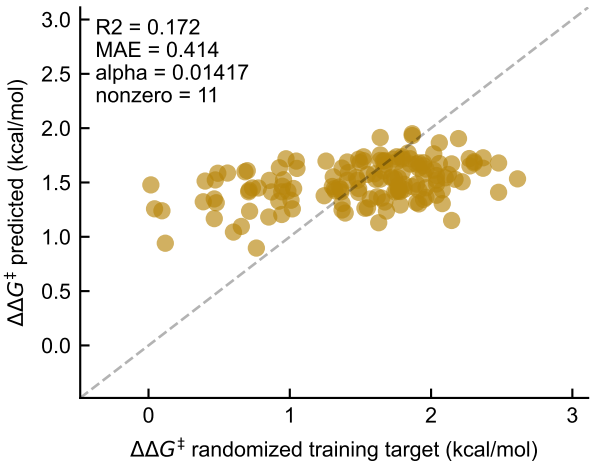
Best training-R2 y-randomized model #15
