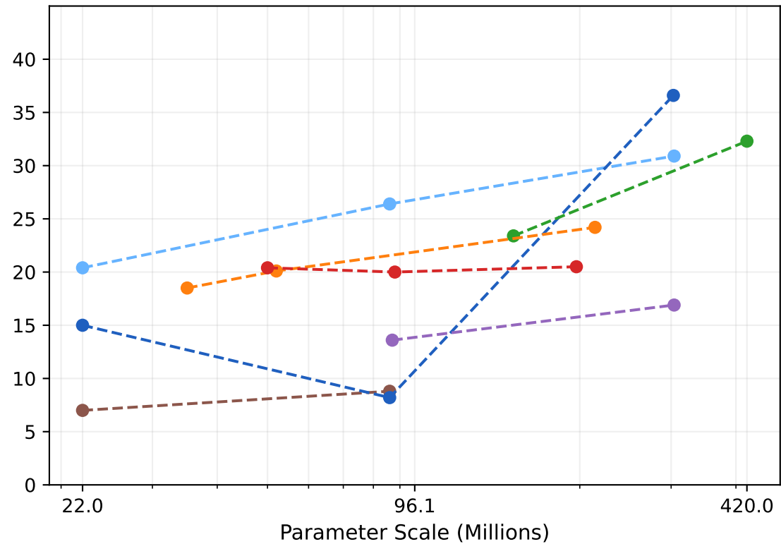
Multi-Color Dataset
