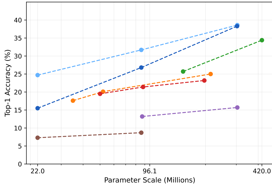
Multi-Factor Dataset
