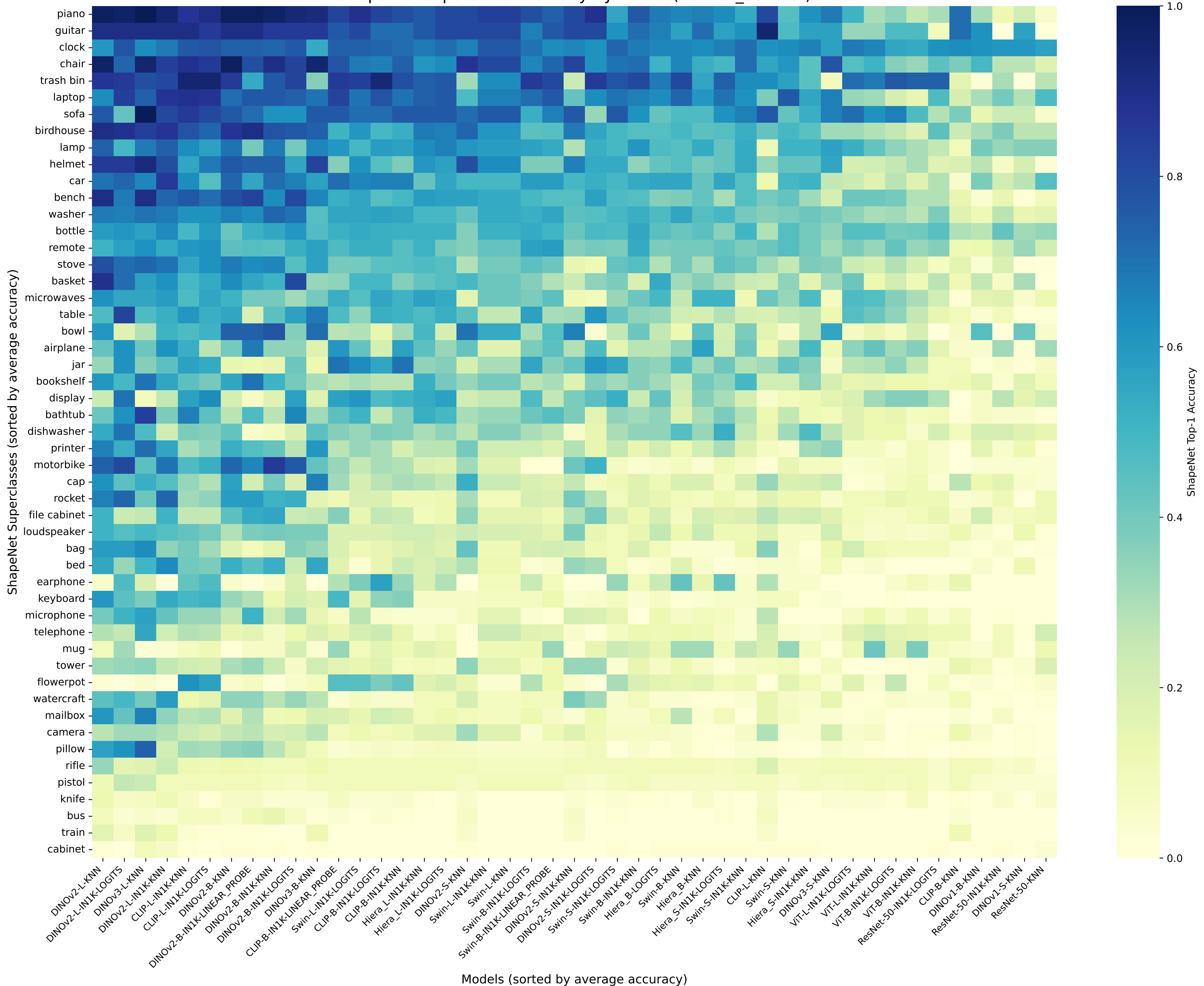
ShapeNet Superclass Accuracy by Model (normal_dataset)
