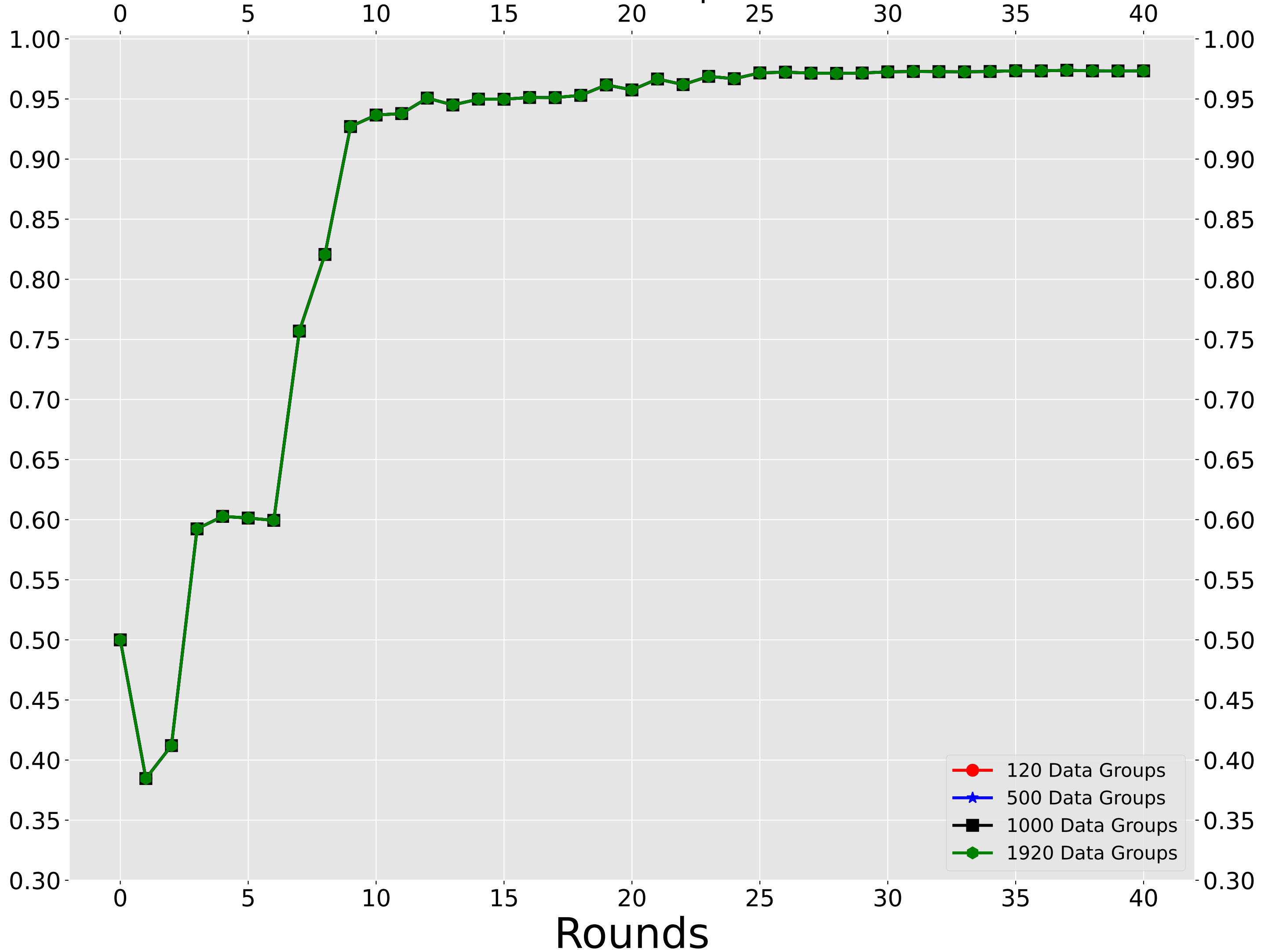
8 Attack 120 -> 1920 Data Groups - Detection Precision
