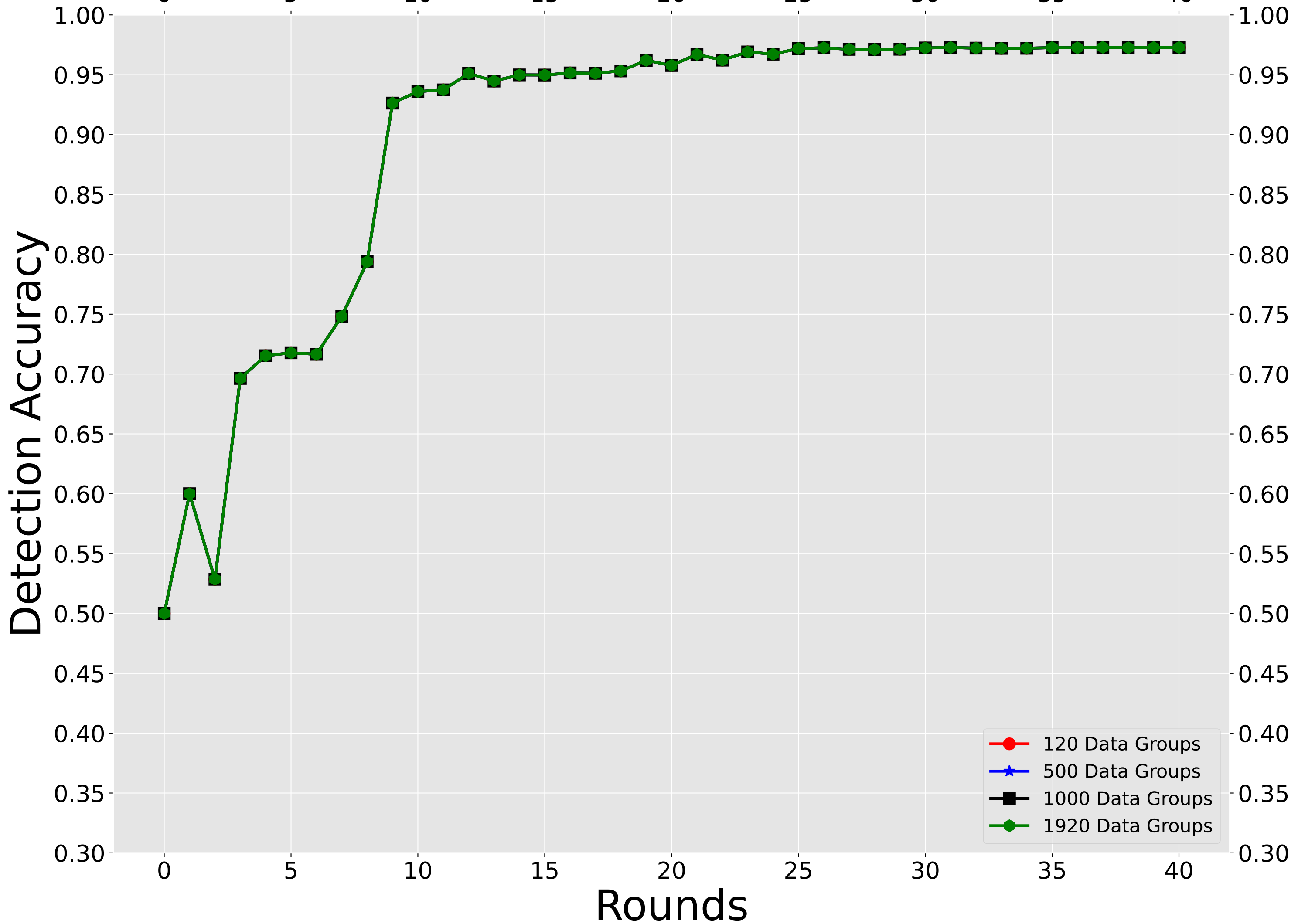
8 Attack 120 -> 1920 Data Groups - Detection Accuracy
