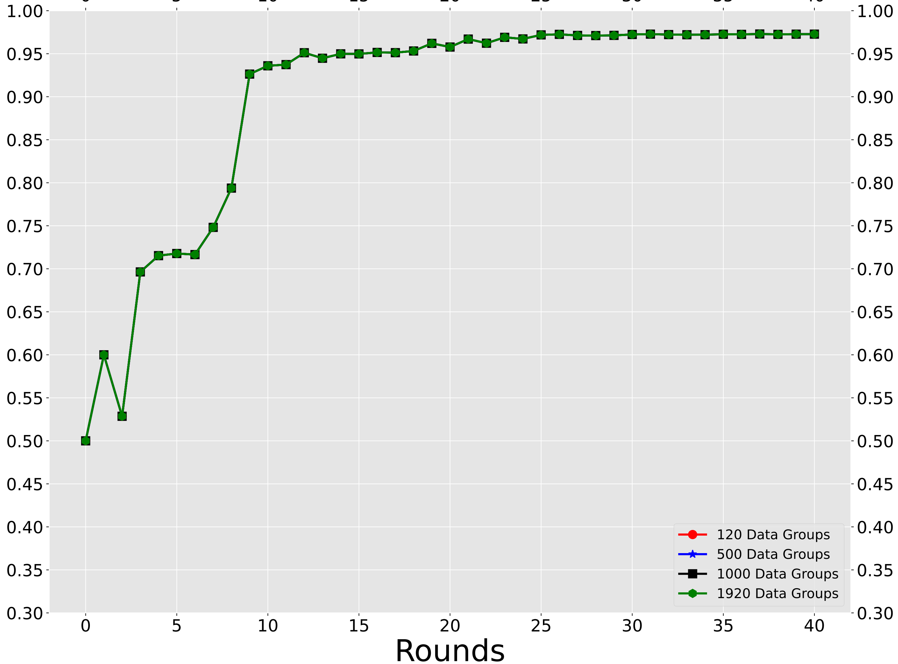
8 Attack 120 -> 1920 Data Groups - Detection Recall
