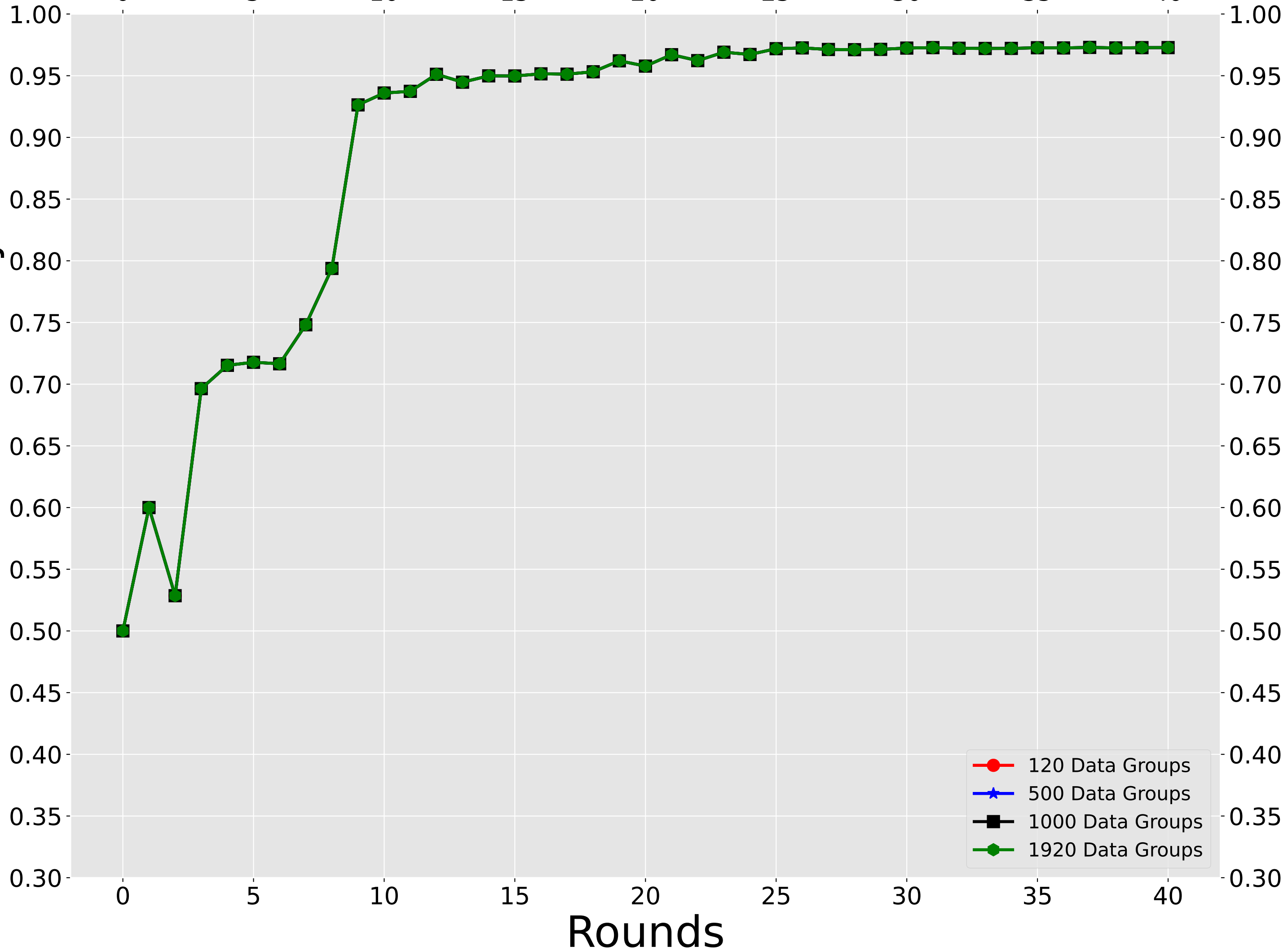
8 Attack 120 -> 1920 Data Groups - Accuracy
