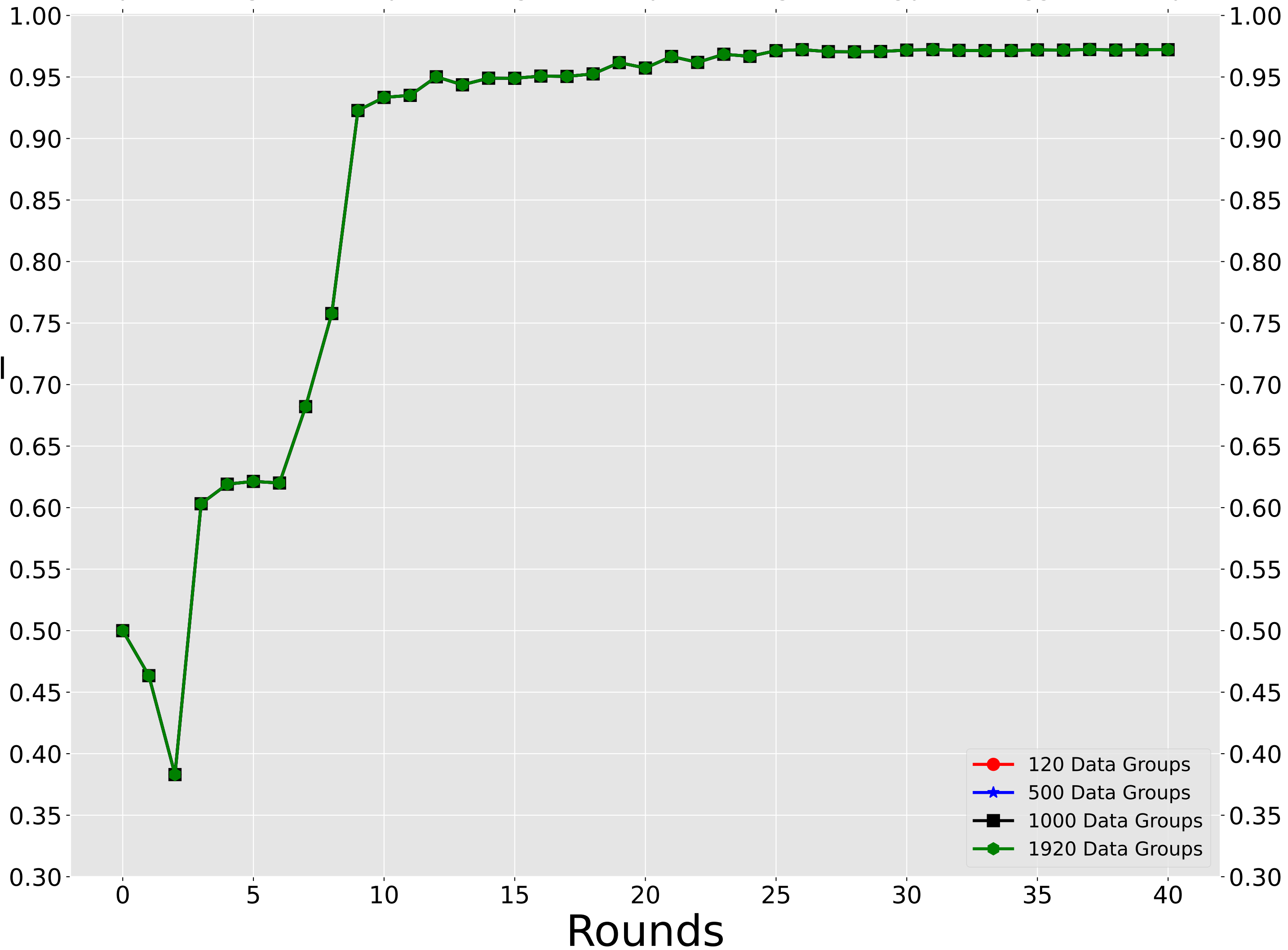
8 Attack 120 -> 1920 Data Groups - Detection F1_Score
