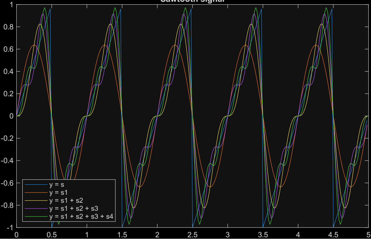
Sawtooth signal
