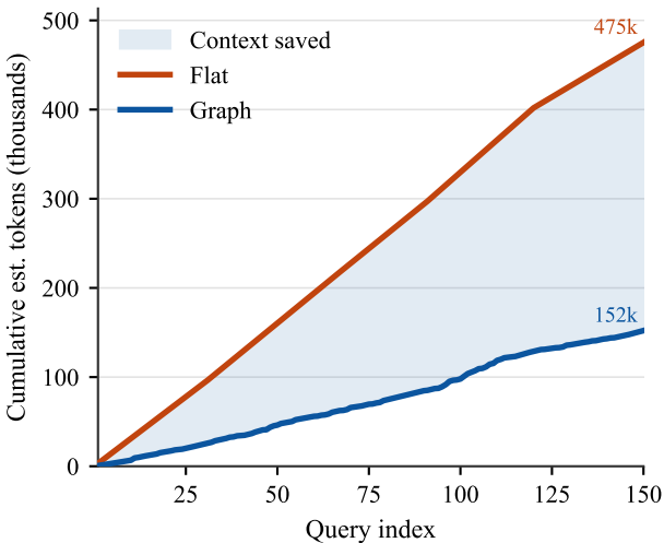
Cost accumulates over 150 queries
