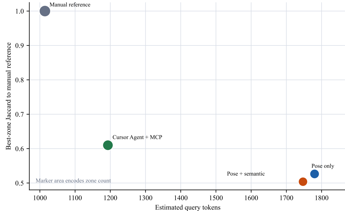
Structure agreement versus query context
