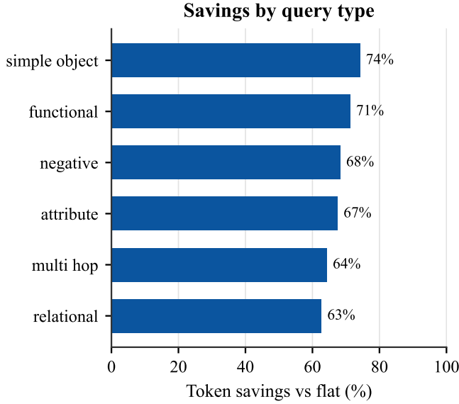
Figure 3: Graph token savings relative to flat, by query type (25 queries each). Hierarchy helps most when a query localizes to a single branch and least when it spans entities or relations across branches.
