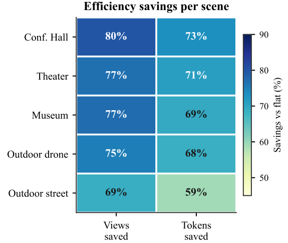
Figure 4: Per-scene efficiency savings (view and token reduction vs. flat, darker = larger saving). Graph traversal lowers query-time cost in every scene, with smaller savings on the noisier outdoor street capture.
