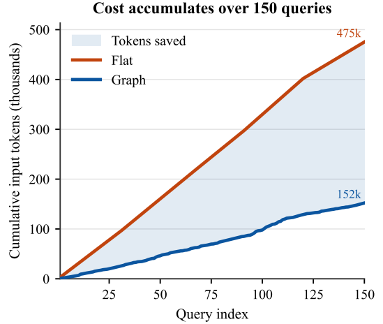
Figure 2: Cumulative input tokens over the 150-query benchmark. The flat baseline grows almost linearly, while graph traversal stays far below; the shaded region is the accumulated saving (475k vs. 152k tokens overall).
