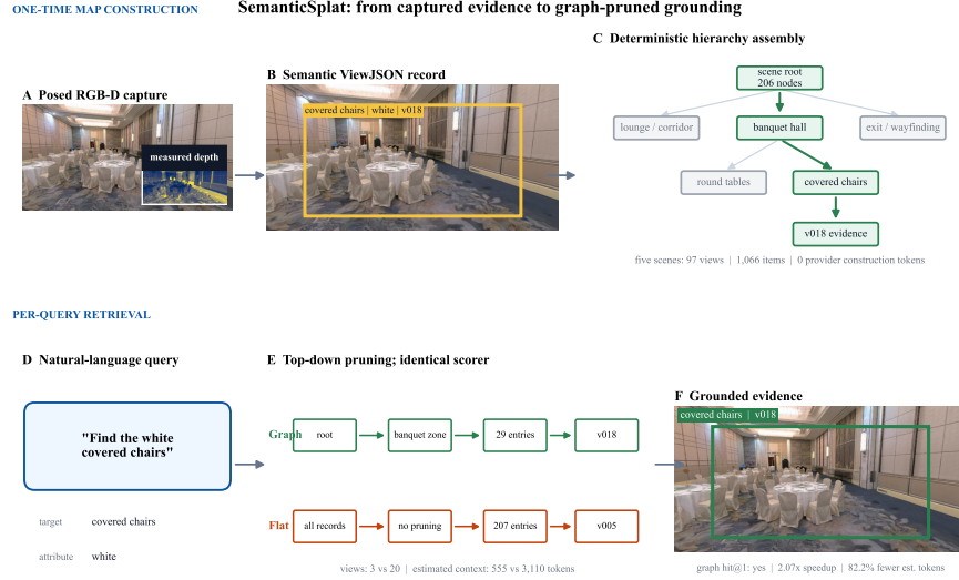
Fig. 1: SemanticSplat end to end, rendered from project evidence rather than illustrative assets. Top: the captured Conference Hall v018 RGB-D observation, its manual ViewJSON record and coarse depth-projected box, and a slice of the checked-in hierarchy. Bottom: saved query qv2_010 is evaluated with the same scorer under graph pruning and flat search, then linked to its returned view. Context-token values are deterministic text-size estimates, not API billing.
