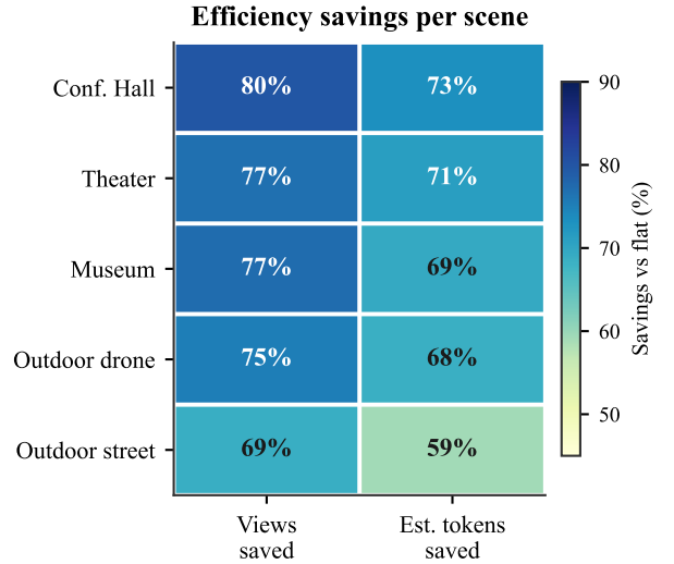
Figure 6: Left: estimated context savings by query type. Right: per-scene view and token reduction. Hierarchy helps most when a query localizes to one branch.
