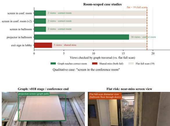
Figure 9: Top: graph views checked versus a 19-view flat scan. Bottom: grounded screen evidence and a flat-scan distractor.
