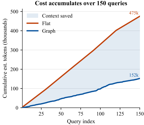
Figure 7: Cumulative estimated context over the 150-query internal benchmark.
