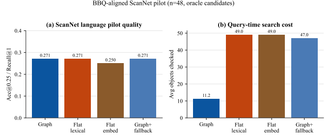
Figure 8: ScanNet oracle-map pilot ( n = 48 ). Graph preserves flat-lexical Acc@0.25 while reducing objects and context; fallback approaches flat cost.
