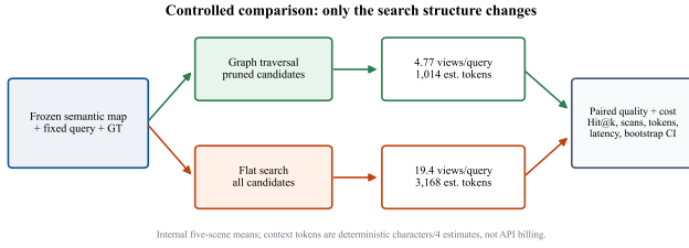
Figure 3: Evaluation tracks. A fair graph-vs.-flat comparison shares maps, queries, labels, and scorer; native external executions have different inputs and do not enter the same ranking.
