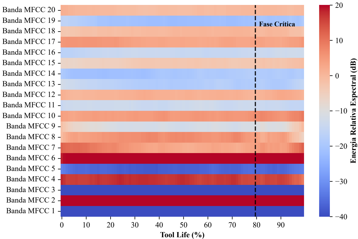
Average MFCC Energy Evolution Across All Drills (Microfone Ultrassônico)
