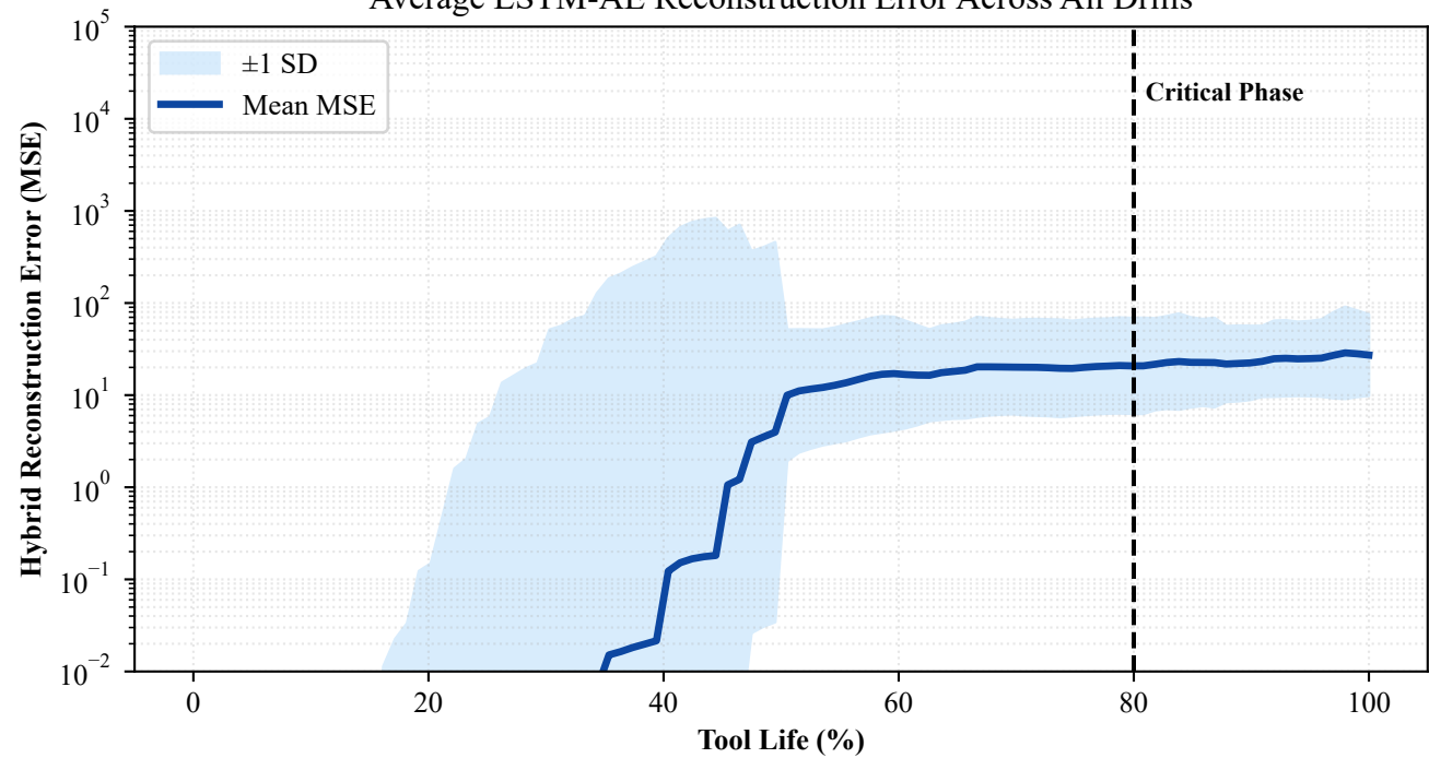
Average LSTM-AE Reconstruction Error Across All Drills
