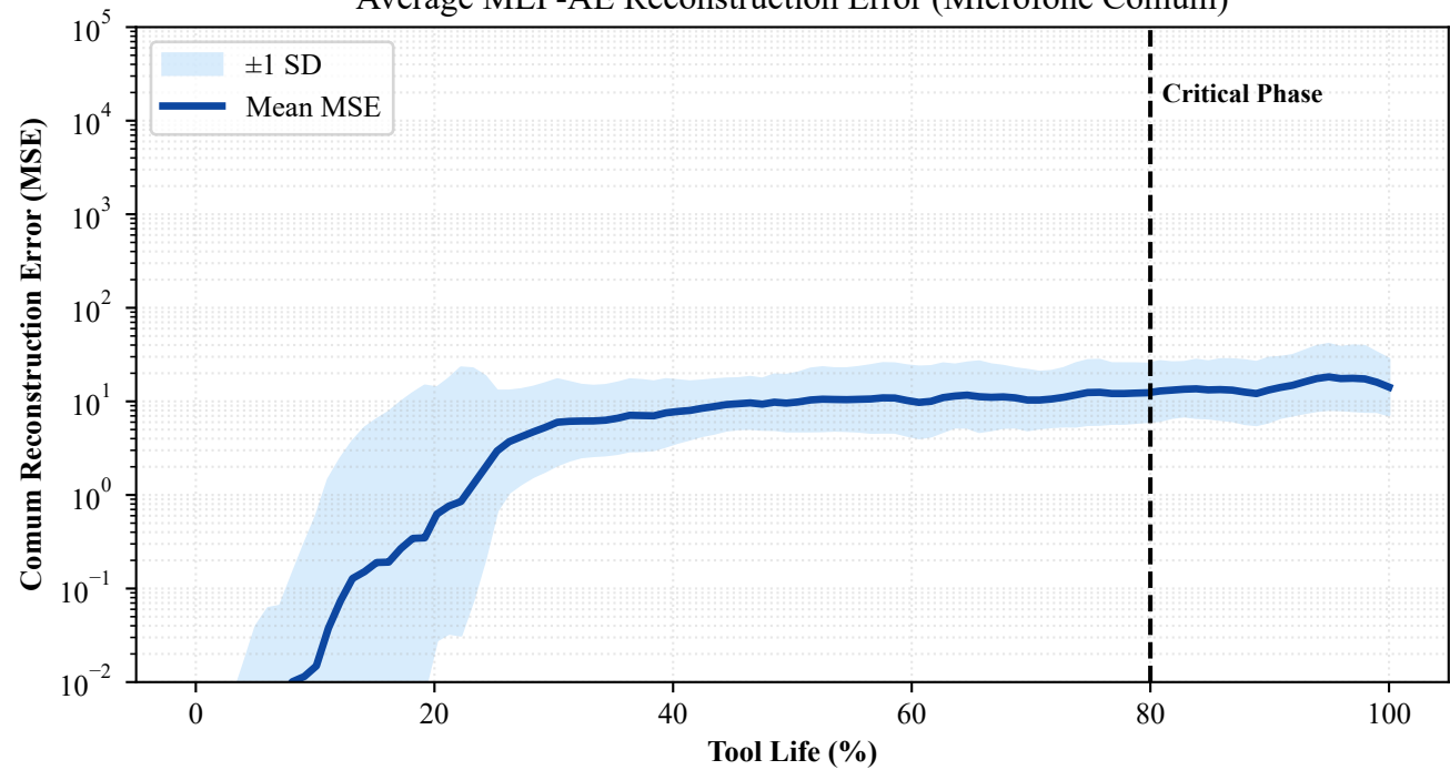
Average MLP-AE Reconstruction Error (Microfone Comum)
