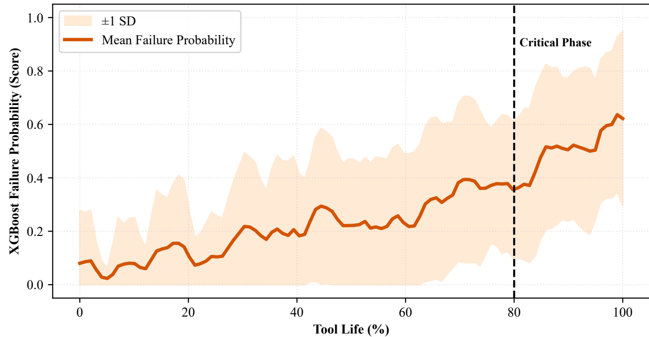
Average XGBoost Failure Probability Across All Drills
