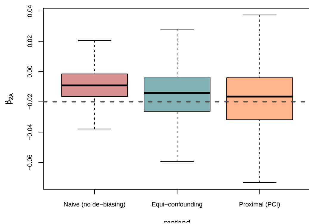
Multiplicative (PCI approximate) -- Equi-confounding violated
