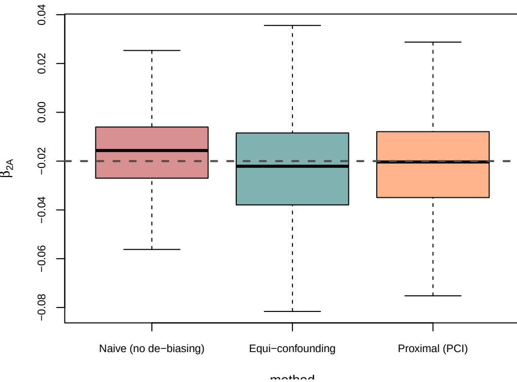
Multiplicative (PCI approximate) -- Equi-confounding holds
