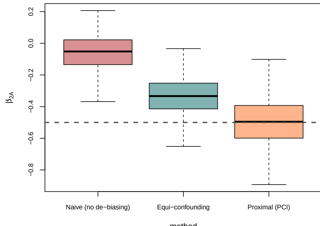
Multiplicative (PCI approximate) -- Equi-confounding violated
