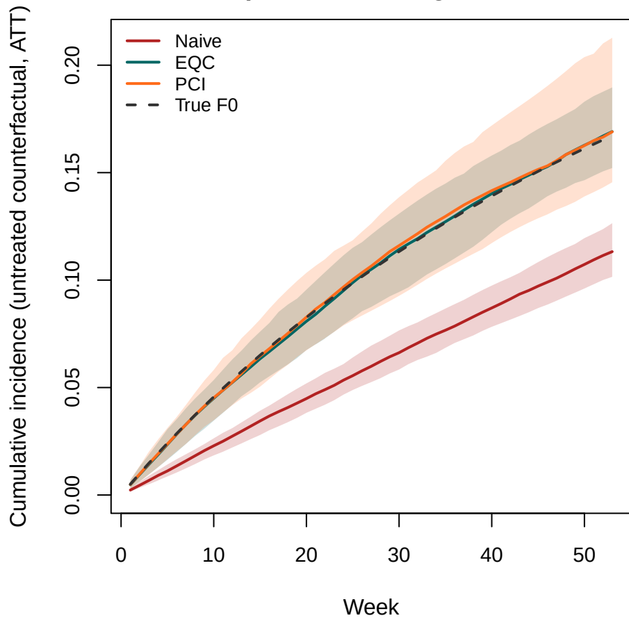
Equi-confounding holds
