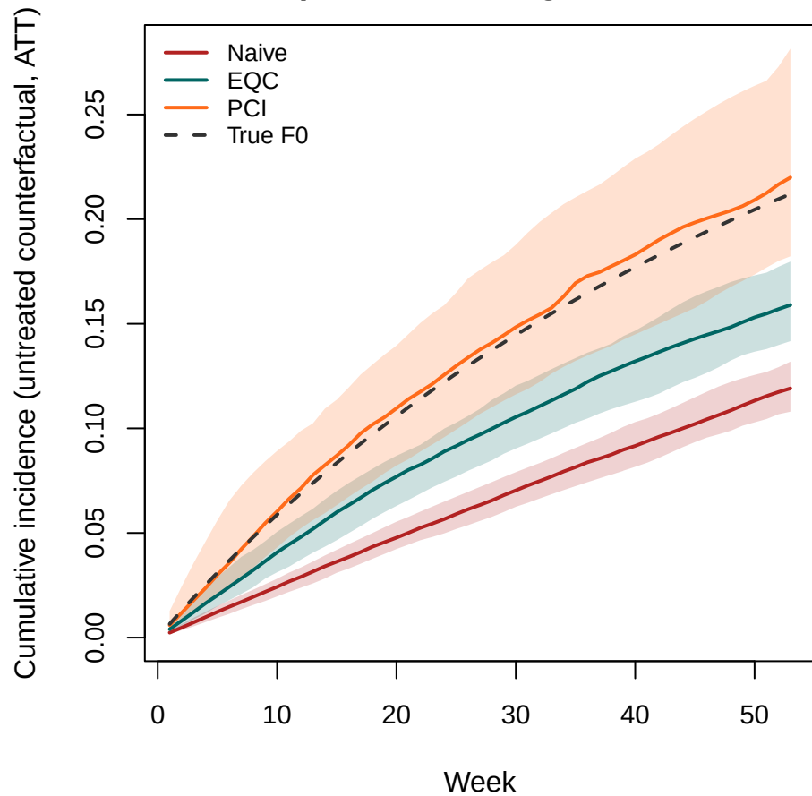
Equi-confounding violated
