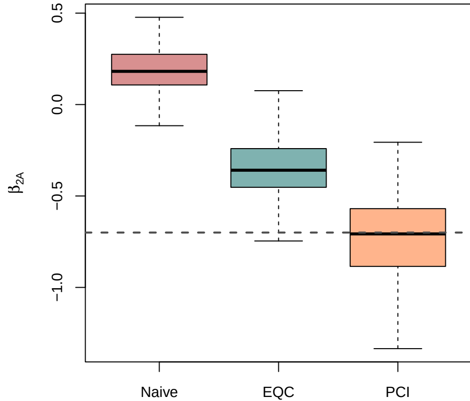
Equi-confounding violated
