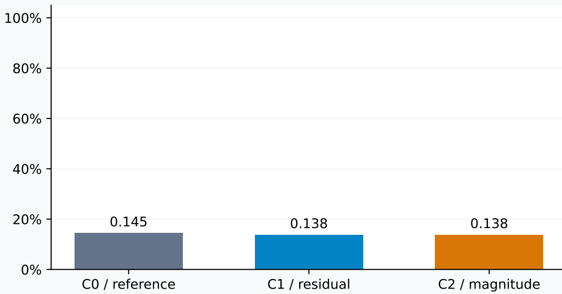
Detector recall
