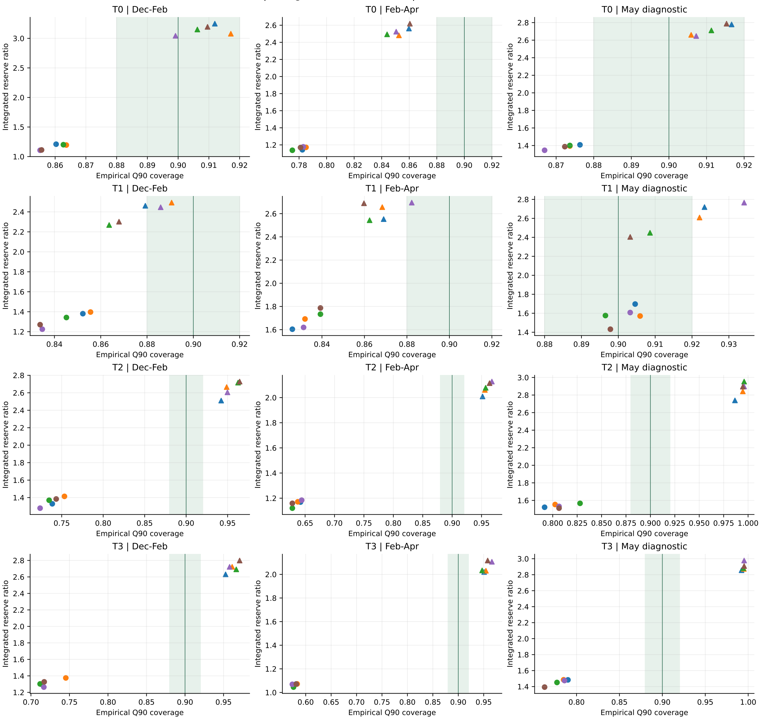
CC4-v2.7: calibration and sharpness Circles: raw | triangles: fixed calibration | F3 = F0 (state unavailable)
